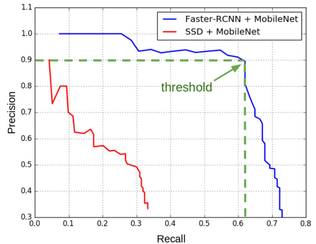
FIGURE 24 Precision recall curve for object detection. The results are tested on the filming testing data, which contains many challenging cases. R-CNN, R-convolutional neural network; SSD, single-shot detector [Color figure can be viewed at wileyonlinelibrary.com]
