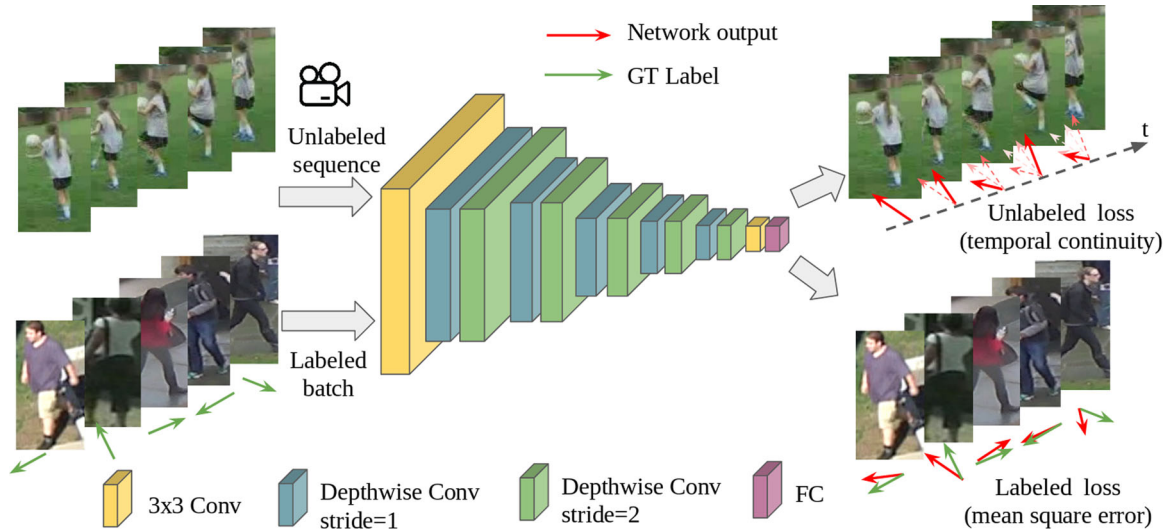
FIGURE 9 Our network architecture for predicting the actor's heading direction. We use a Mobilenet-based feature extractor followed by a convolutional layer and a fully connected layer to regress to angular values. The network is trained using both labeled and unsupervised losses [Color figure can be viewed at wileyonlinelibrary.com ]
