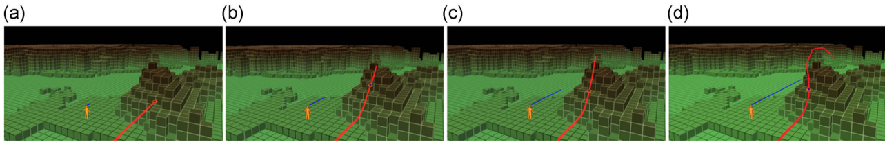
FIGURE 30 Planner behavior with different time horizons of 1 (a), 5 (b), 10 (c), and 20 (d) seconds for the same actor trajectory and environment. The shortest time horizon of 1 s is not sufficient for the planner to find a trajectory that avoids the mound, and the vehicle gets stuck in a bad local minimum of solutions. Longer horizons let the UAV plan more intelligent trajectories, reasoning about obstacle shapes long before the UAV reaches those positions. UAV, unmanned aerial vehicle [Color figure can be viewed at wileyonlinelibrary.com ]
