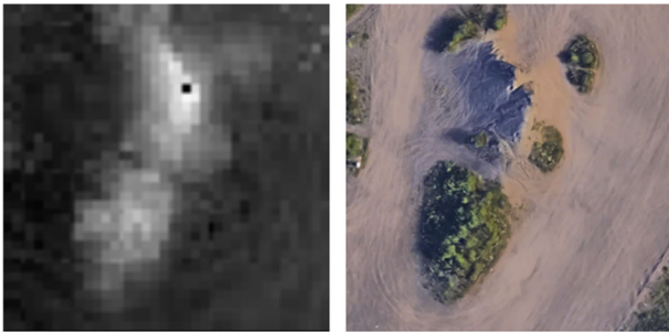
FIGURE 12 The left figure shows the height map accumulated overflight over a small mountain. The color scale goes from 0 (−10 m) to 255 (+10 m), where the zero reference of 127 is taken at the unmanned aerial vehicles initial takeoff height. The right figure is the top-down view of the mountain of the same place [Color figure can be viewed at wileyonlinelibrary.com ]
