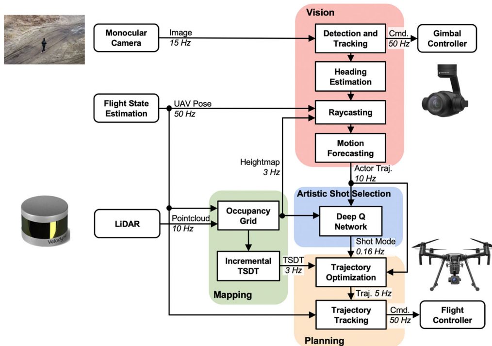
FIGURE 2 The system consists of four main modules running in parallel: Vision, mapping, planning, and artistic shot selection. The system takes in visual, LiDAR, and GPS inputs to output gimbal and flight controller commands [Color figure can be viewed at wileyonlinelibrary.com ]
