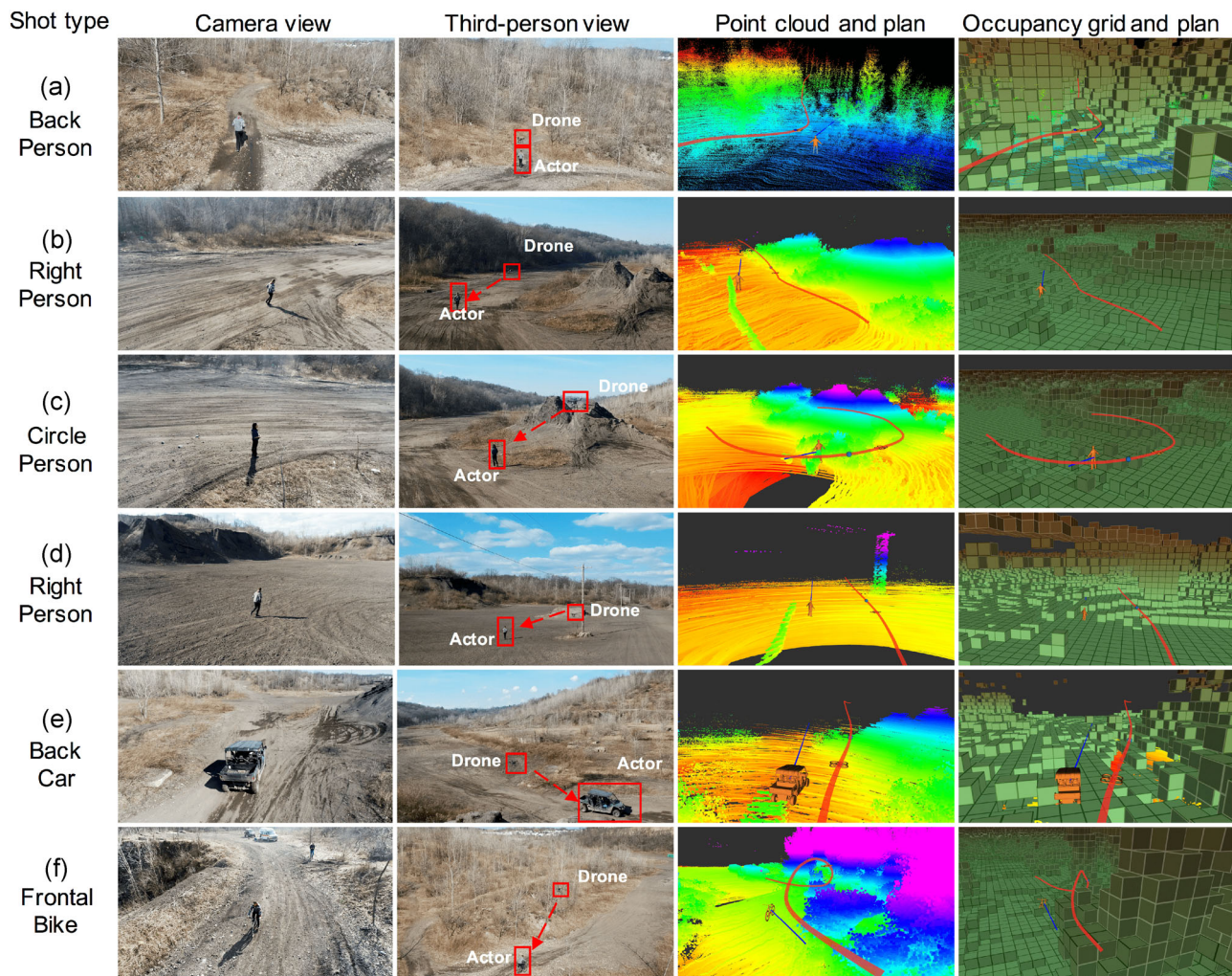
FIGURE 20 Field results with different fixed shot types in multiple environment types, following different actor types. The UAV trajectory (red) tracks the actor's forecasted motion (blue) and stays safe while avoiding occlusions from obstacles. We display accumulated point clouds of LiDAR hits and the occupancy grid: (a) Back shot following runner in narrow tree trail; (b) Right-side shot following a runner close to dirt mound; (c) Circular shot on person close to dirt mound; (d) Right-side shot below the 3D structure of an electric wire. Note that LiDAR registration is noisy close to the pole in a row due to large electromagnetic interference with the UAV's compass; (e) Right-side shot following car close to dirt mound; (f) Frontal shot on biker going downhill on a trail with tall trees. UAV, unmanned aerial vehicle [Color figure can be viewed at wileyonlinelibrary.com ]
