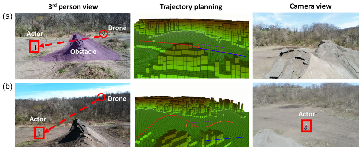
FIGURE 31 Comparison of planning (a) without and (b) with occlusion cost function in a special setup where actor positioning comes from a GPS tag. The occlusion cost function significantly improves the quality of the camera image in comparison with pure obstacle avoidance, for same shot type [Color figure can be viewed at wileyonlinelibrary.com ]
