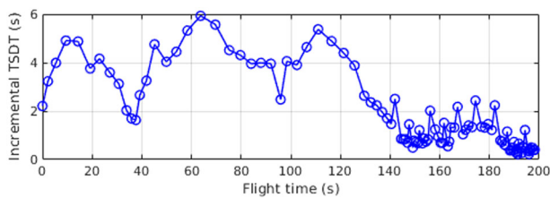
FIGURE 22 Incremental distance transform computation time over flight time. The first operations take significantly more time because of our map initialization scheme where all cells are initially considered as unknown instead of free, causing the first laser scans to update a significantly larger number of voxels than later scans. During calculation the planner is not blocked: it can still access TSDT values from the latest version of \mathcal{M} . TSDT, truncated signed distance transform [Color figure can be viewed at wileyonlinelibrary.com ]
