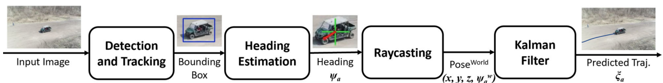
FIGURE 5 Vision subsystem. We detect and track the actor's bounding box, estimate its heading, and project its pose to world coordinates. A Kalman filter predicts the actor's forecasted trajectory \zeta_a [Color figure can be viewed at wileyonlinelibrary.com ]
