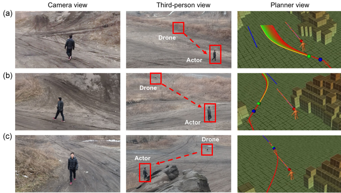
FIGURE 37 UAV follows an actor while switching shot types autonomously with our trained policy: (a) UAV starts at the back of the actor; (b) The mound's presence on the right-side of the actor leads to a left shot selection; (c) UAV switches to a frontal shot in the open area. UAV, unmanned aerial vehicle [Color figure can be viewed at wileyonlinelibrary.com ]
