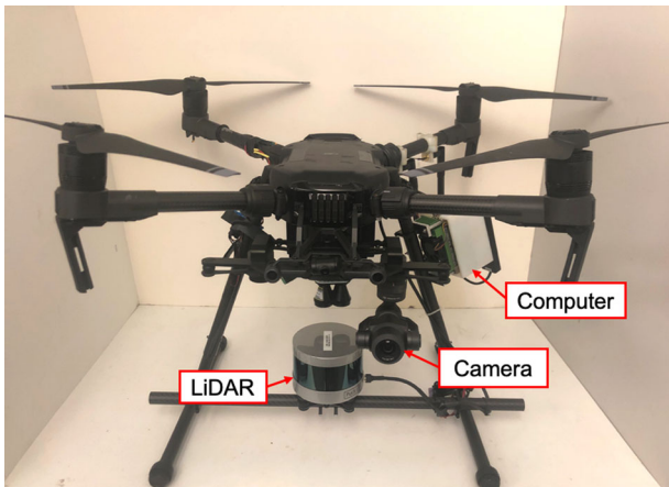
FIGURE 3 System hardware: DJI M210 drone equipped with Nvidia TX2 computer, Velodyne VLP-16 Puck Lite LiDAR and Zenmuse X4S camera gimbal [Color figure can be viewed at wileyonlinelibrary.com]
