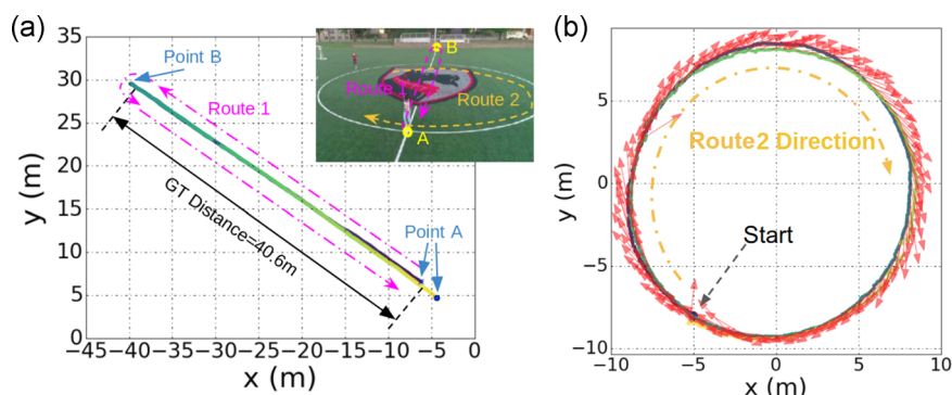
FIGURE 27 Pose and heading estimation results. (a) Actor walks on a straight line from points A-B-A. Ground-truth trajectory length is 40.6 m, while the estimated motion length is 42.3 m. (b) The actor walks along a circle. Ground-truth diameter is 18.3 m, while the estimated diameter from ray-casting is 18.7 m. Heading estimation appears tangential to the ground circle [Color figure can be viewed at wileyonlinelibrary.com ]
