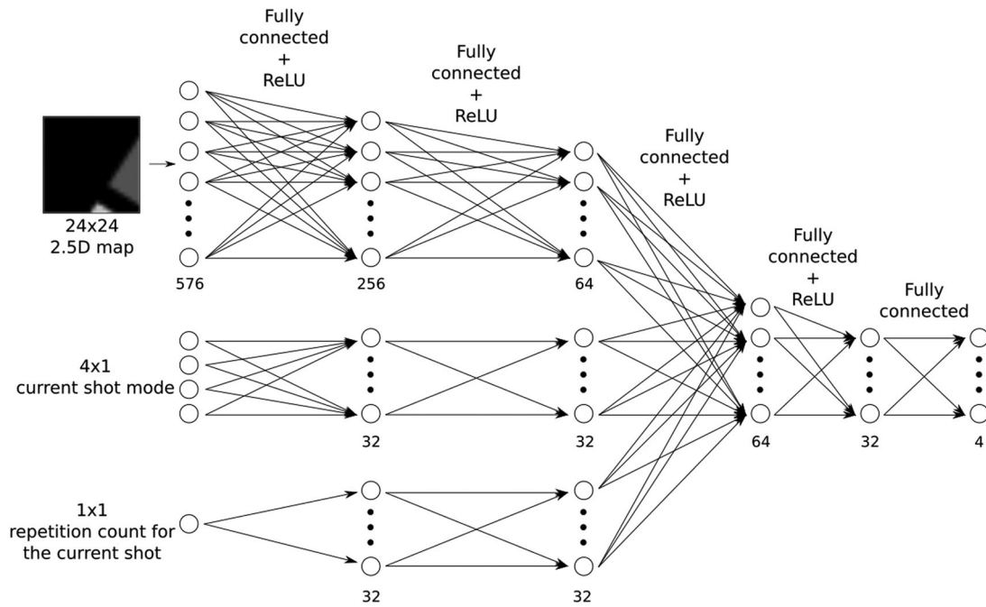
FIGURE 18 DQN architecture consisting of fully connected layers. Each portion of state is first fed to separate mini-networks of two layers. Then, the outputs of these are combined in three consecutive layers whose output is the Q values
