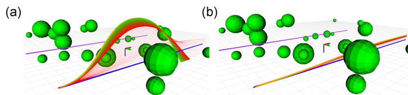
FIGURE 32 A randomized environment with obstacles to evaluate planner robustness. Unmanned aerial vehicle trajectory initialization shown in blue, actor trajectory in purple, and planner iterations vary from red to green (final solution). (a) Solution including occlusion cost function and (b) pure obstacle avoidance [Color figure can be viewed at wileyonlinelibrary.com ]
