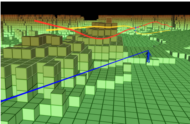
FIGURE 28 Performance comparisons between planning with full knowledge of the map (yellow) vs. with online mapping (red), displayed over the ground truth map grid. Online map trajectory is less smooth due to imperfect LiDAR registration and new obstacle discoveries as the flight progresses [Color figure can be viewed at wileyonlinelibrary.com]
