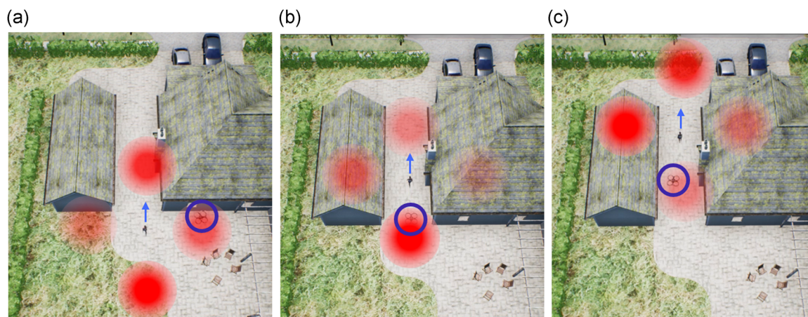
FIGURE 35 Visualization of the Q values of the DQN during testing corresponding to the four shot types. The more opaque a circle is, the higher is the action’s Q value. The drone position before each decision is indicated by a blue ring around the drone. The drone starts on the right side of the actor and switches to back shot mode to traverse a narrow passage (a) where it stays in the actor’s back for one-time step (b). Finally, it decides to switch to a left-side shot once the obstacles are passed (c) [Color figure can be viewed at wileyonlinelibrary.com ]
