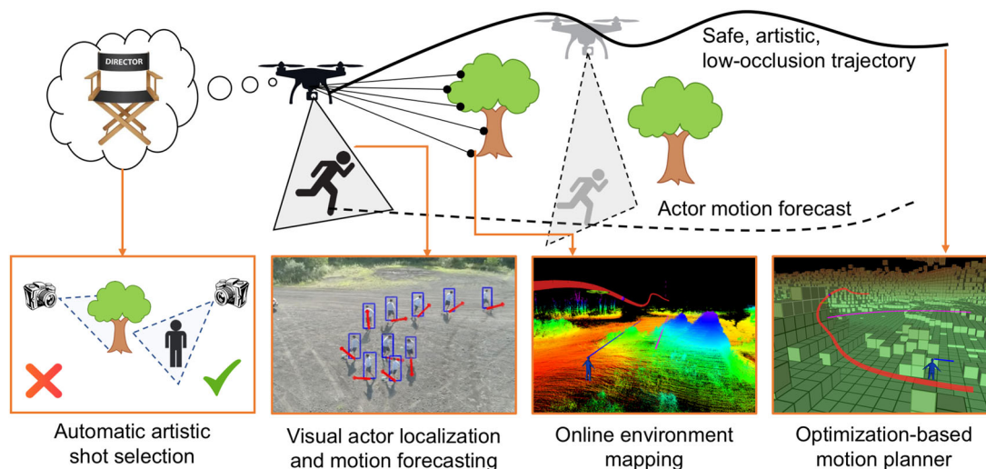
FIGURE 1 Aerial cinematographer pipeline: the unmanned aerial vehicle visually detects the actor's motion using a vision-based localization module, maps the environment with an onboard LiDAR sensor, reasons about artistic guidelines, and plans a smooth, collision-free trajectory while avoiding occlusions [Color figure can be viewed at wileyonlinelibrary.com ]
