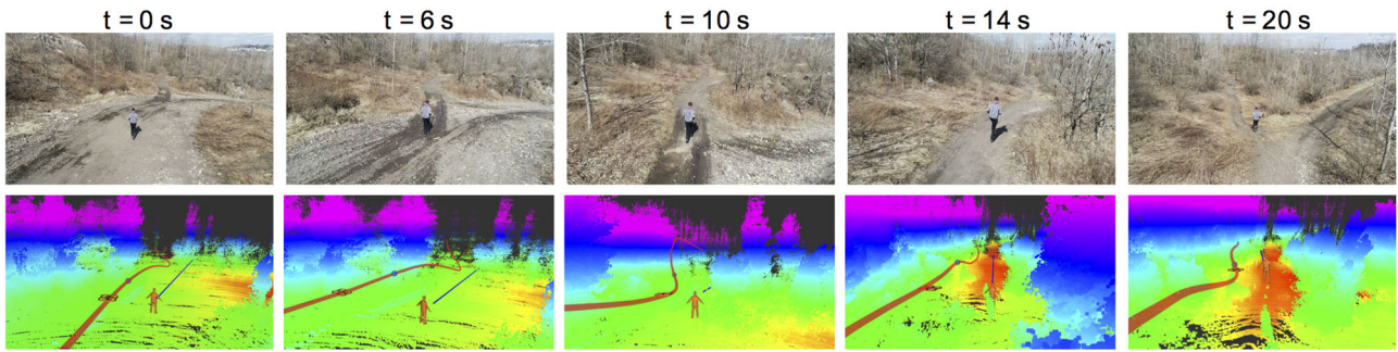
FIGURE 21 Detailed time-lapse of back shot following a runner in a narrow trail with trees. As the unmanned aerial vehicle approaches the trees at t = 6 s, the trajectory bends to keep the vehicle safe, maintain target visibility, and follow the terrain's downward inclination [Color figure can be viewed at wileyonlinelibrary.com ]
