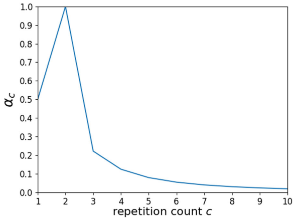
FIGURE 16 Values of the variable discount parameter \alpha_c over shot repetition count c [Color figure can be viewed at wileyonlinelibrary.com]
