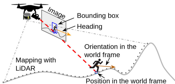
FIGURE 10 Ray-casting module uses the actor's bounding box, estimated heading angle, environment height map, and camera matrices to obtain pose of the actor in the world frame [x, y, z, \psi_a^w] [Color figure can be viewed at wileyonlinelibrary.com ]
