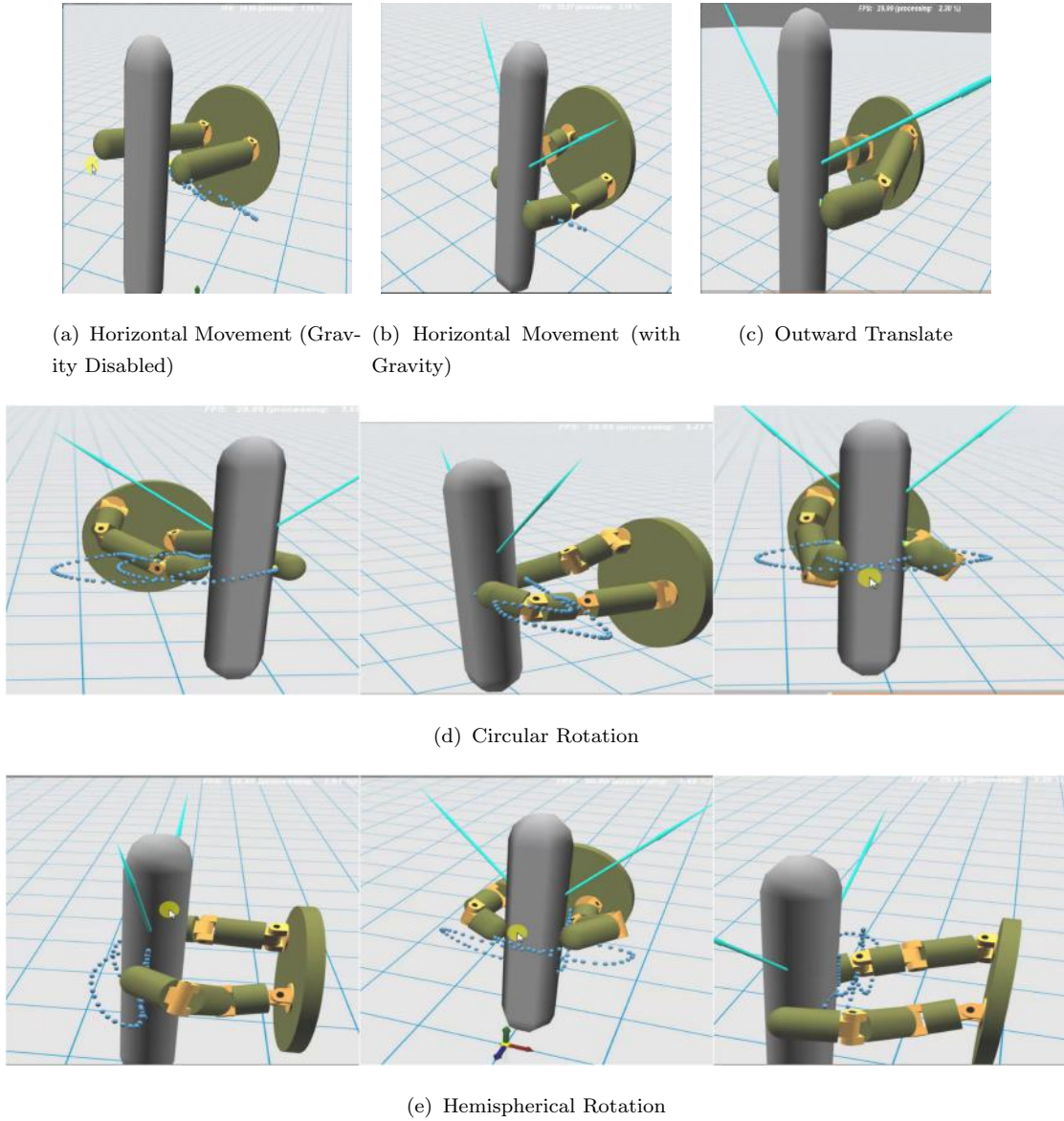
FIGURE 3.6: In this set of examples, we build up a 2 finger gripper by specifying an increasingly complex set of objectives, creating an increasingly complex set of floating motion plans. The optimization builds more capable versions of these manipulators as needed to follow the required trajectories and actively supply the necessary force. We can also view the later hand designs in this sequence as multi-objective hands, since they can accomplish multiple distinct primitive motions (which happen to be chained together).
