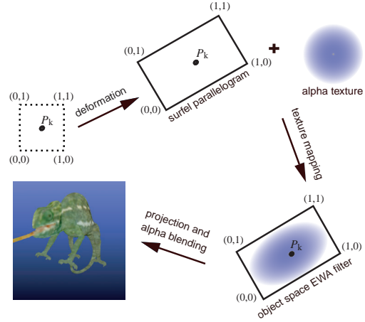
Figure 6: EWA splatting using textured polygons. Note the dashed line means the shape of the surfel polygon can not be determined before rendering, but is view dependent.
