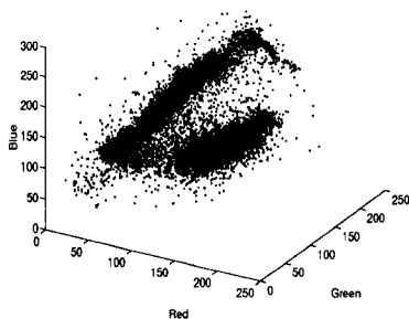
Figure 3. Color space for a typical road scene.
