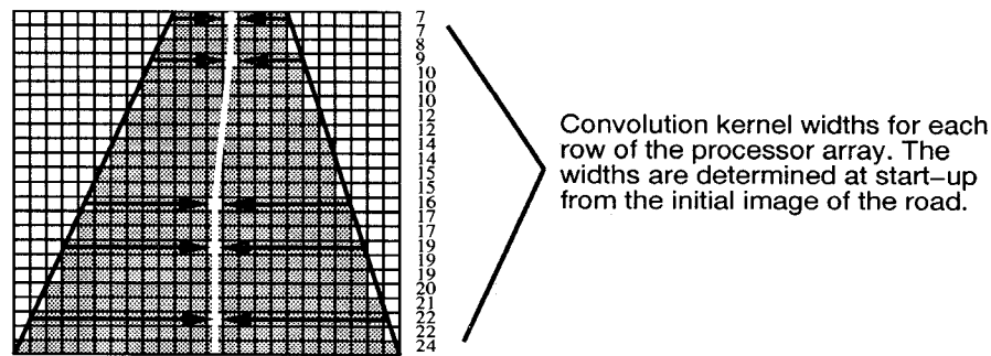
Figure 8. Convolution kernels for different rows centered on the actual center line of the road superimposed on the processor array. Arrows indicate the direction of travel of the convolution summation.
