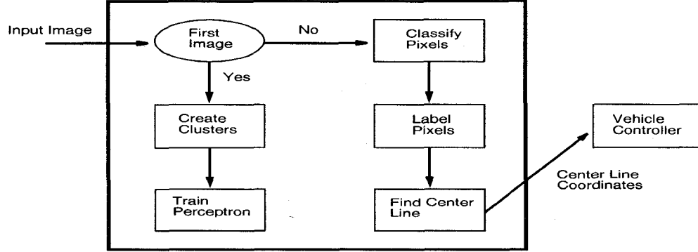
Figure 2. Block diagram of system architecture. Steps located inside the large black box are computed in parallel on the processor array.
