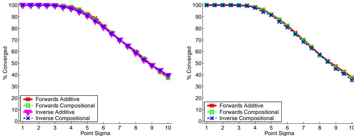
(a) Frequency of Convergence for Affine Warps (b) Frequency of Convergence for Homographies
