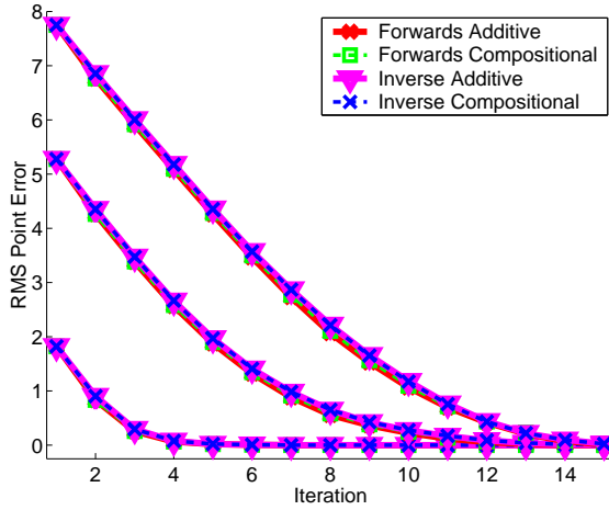
(c) Average Convergence Rates for “Knee” image
