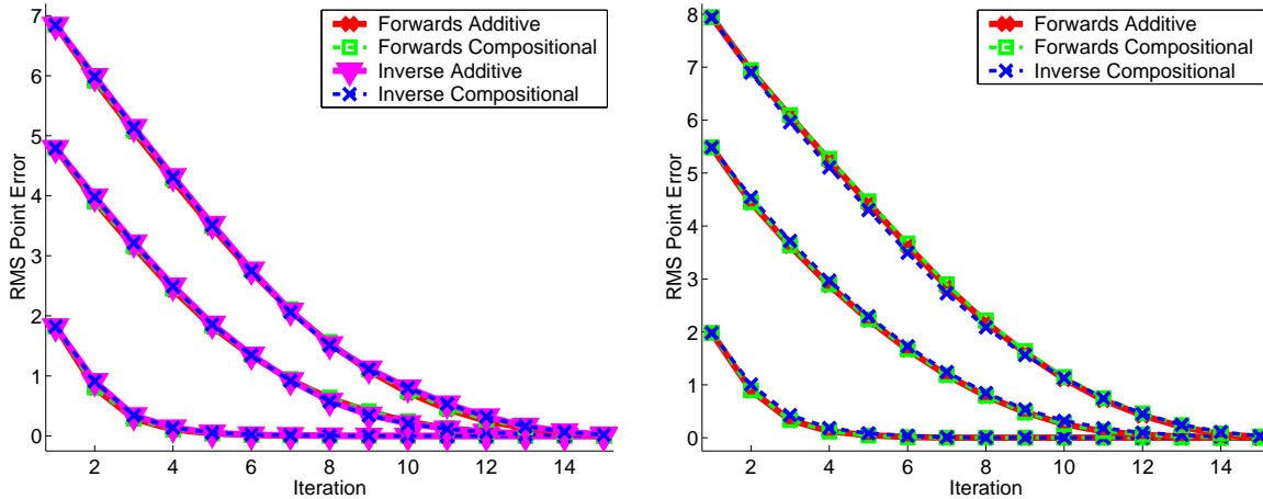
(a) Average Convergence Rates for Affine (b) Average Convergence Rates for Homography
