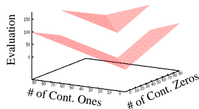
Figure 2: Two Views of the same four peaks problem. As T increases, the area in the upper triangle decrease.
