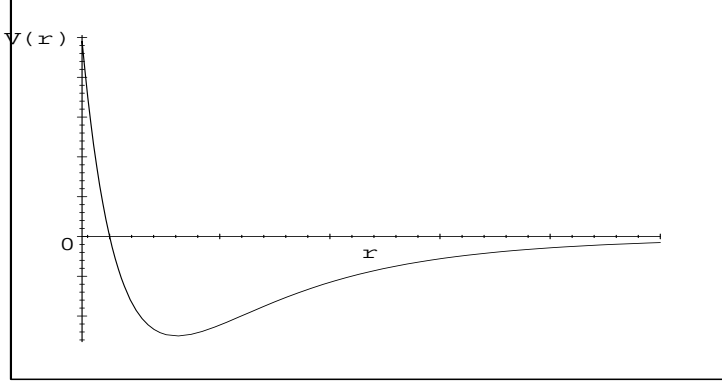
Fig. 3. A typical one-dimensional Lennard-Jones potential-well
