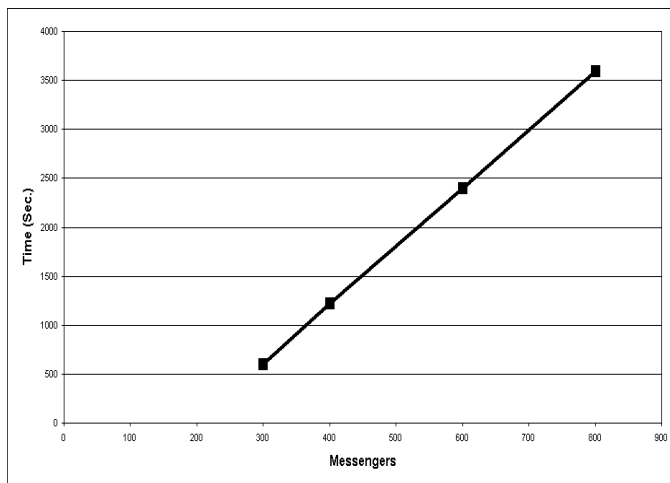
Fig. 11. The time for an agent to reach a task (y axis) increases as the number and density of agents in the system (x axis) increases.
