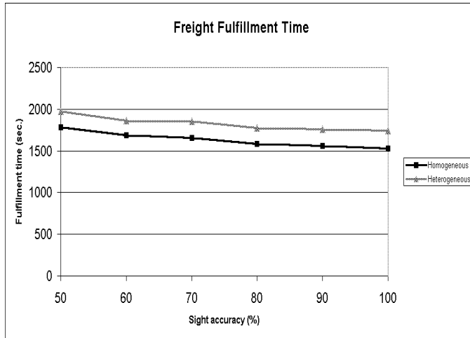
Fig. 14. The average time for task allocation and execution (y axis) decreases as the accuracy of message reception (x axis) increases.
