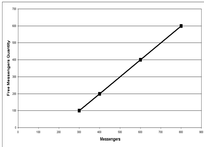
Fig. 9. The number of messengers moving towards freights (y axis) as a function of the number of messengers in the system (x axis). Other agents perform tasks concurrently.
