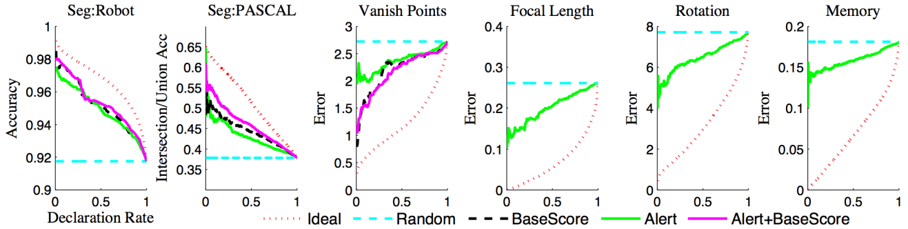
Figure 3: Accuracy or Error of BASESYS vs. Declaration Rate Curves. We used accuracy and intersection/union for evaluating segmentation (robot and PASCAL respectively), and the mean of three errors for vanishing point estimation. Results for other choices of y_i described in Section 3 can be found on author’s webpage. Results are averaged over 10 random train/test splits. BASESCORE is not shown for focal length, rotation and memorability prediction because the first two are direct products of vanishing point estimates, and the inner workings of BASESYS for the latter do not lead to an obvious definition for BASESCORE. Best viewed in color.
