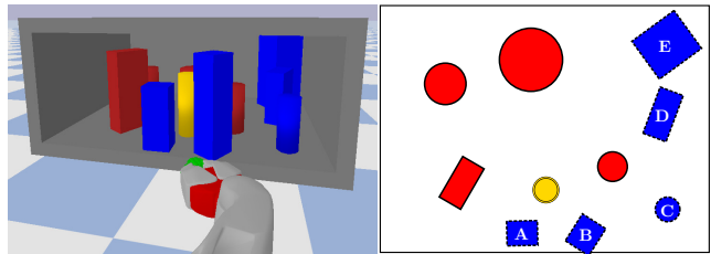
Figure 2: MAMO workspace (left) and its 2D projection labelled with movable object IDs. Movable objects are in blue, immovable obstacles in red, and the object-of-interest to be retrieved in yellow.
