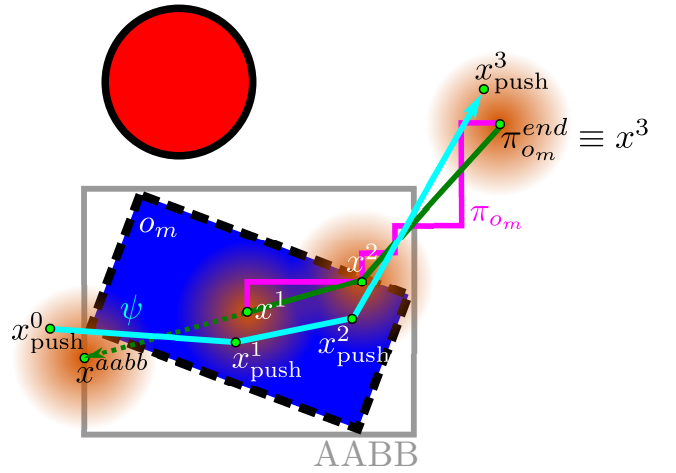
Figure 5: 2D illustration of our push planner. Given a movable object o_m (blue) and its MAPF solution path \pi_{o_m} (pink), we shortcut \pi_{o_m} while accounting for immovable obstacles \mathcal{O}_I (red) to get the green path of straight line segments. After computing x^{aabb} by intersecting the \overline{(x^2, x^1)} ray with the axis-aligned bounding box for o_m , the push action (cyan) is computed via inverse kinematics between sampled points x_{\text{push}}^i \sim \mathcal{N}(x^i, \sigma I) , i = \{0, \dots, n\} , x^0 := x^{aabb} .
