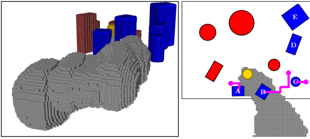
Figure 3: The negative goal region (NGR) \mathcal{V}(\hat{\pi}_{\mathcal{R}}) in gray for the MAMO problem from Fig. 2. (left) 3D volumes of the NGR and all objects at their initial poses (we omit the shelf for ease of visualisation). (right) 2D projection of the NGR and the workspace, overlaid with the solution to the abstract MAPF problem formulated for this scene. Objects A and B need to move outside the NGR, and object C needs to move to allow A to reach its goal. MAPF solution paths are shown in pink.
