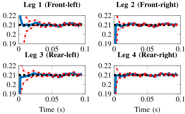
Fig. 4. The calf length estimation result using simulation data. \rho = [l_c] . In all plots, blue lines are estimated length. Red dash lines show the 3\sigma uncertainty envelope. Black dash lines indicate the ground truth length 0.21 m for reference. All estimations converge to ground truth quickly with final errors < 0.01 m.
