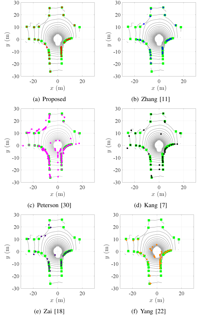
Fig. 10. Comparison results of the curb detection method in Scenario (d).
