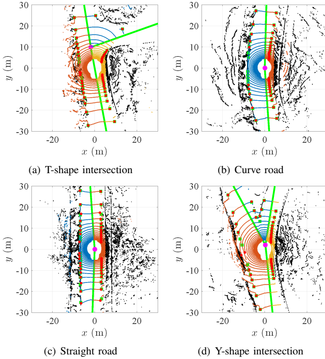
Fig. 9. Examples of the curb detection method.
