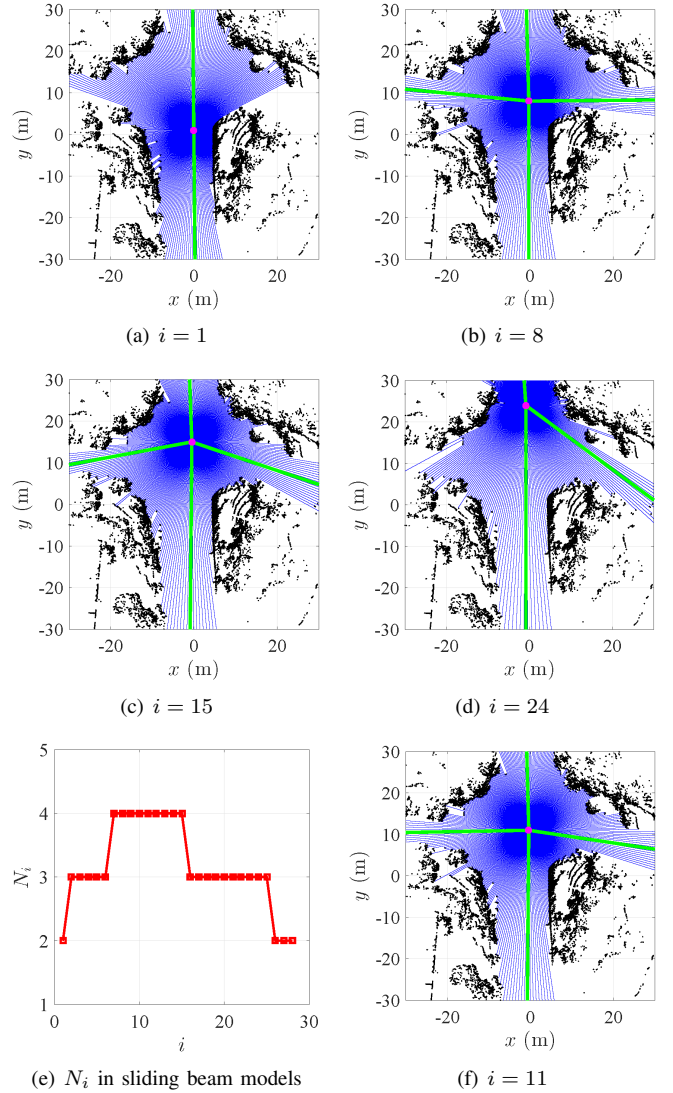
Fig. 6. An example of the top-layer beam model. The sliding beam transferred from the current position of the vehicle to the edge of the region to detect the segments on road.
