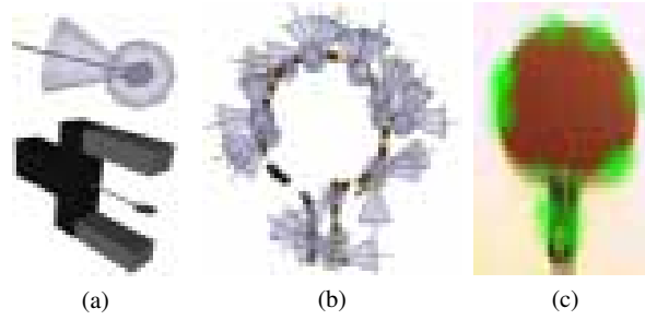
Fig. 16 Grasp density representation. The top image of Fig. (a) illustrates a particle from a non-parametric grasp density and its associated kernel widths: the translucent sphere shows one position standard deviation, the cone shows the variance in orientation. The bottom image illustrates how the schematic rendering used in the top image relates to a physical gripper. Figure (b) shows a 3D rendering of the kernels supporting a grasp density for a table-tennis paddle (for clarity, only 30 kernels are rendered). Figure (c) indicates with a green mask of varying opacity the values of the location component of the same grasp density along the plane of the paddle.
