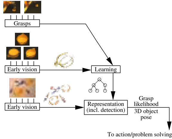
Fig. 11 Overview of learning to grasp. Learning produces graph-structured object representations that combine experienced grasps with visual features provided by early vision. Subsequently, instances can be detected in new scenes provided by early vision. Detection directly produces pose estimates and suitable grasp parameters.
