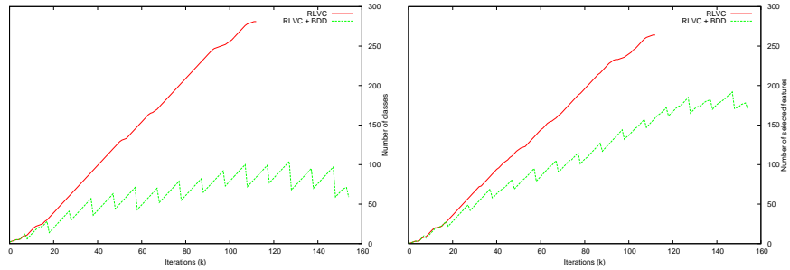
Fig. 9 Comparison of the number of generated classes and selected visual features between the basic and BDD versions of RLVC. The number of visual classes (resp. selected features) as a function of the stage counter k is shown on the left (resp. right). The sawtooth patterns are due to the periodicity of the compaction phases.
