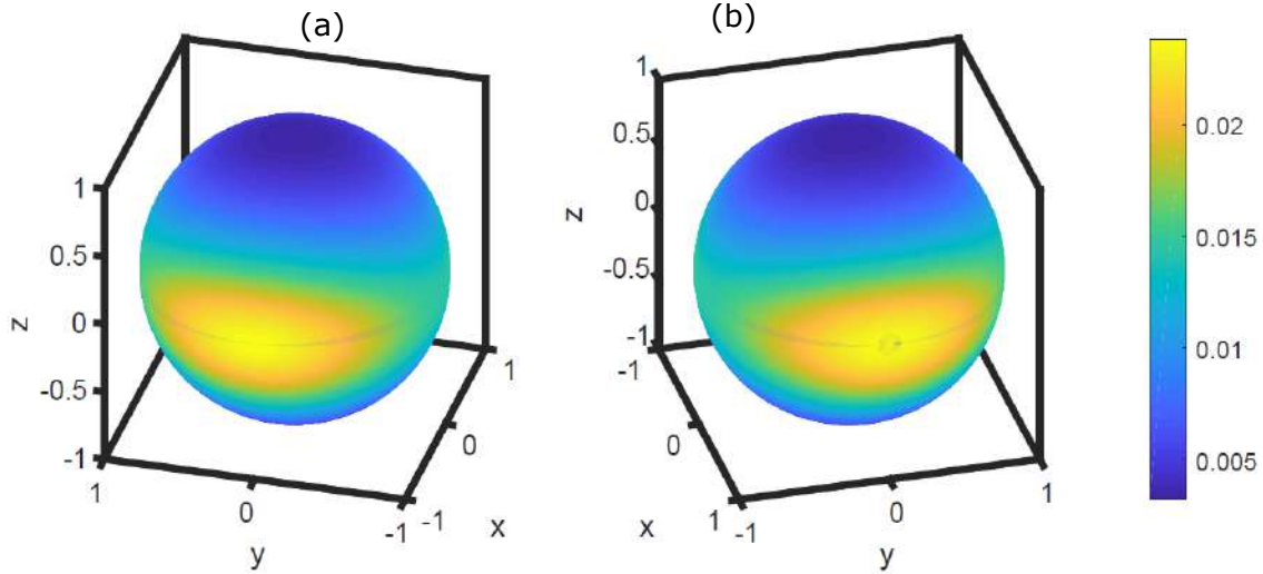
Figure 6-1: A 3D Bingham distribution: c = \frac{1}{N} \exp(\mathbf{v}^T \mathbf{M} \mathbf{Z} \mathbf{M}^T \mathbf{v}) , where \mathbf{M} = \mathbf{I}_{3 \times 3} , \mathbf{Z} = \text{diag}(0, -0.5, -2) , and \mathbf{v} = (x, y, z)^T , \mathbf{v}^T \mathbf{v} = 1 . The colors on the sphere show the probability value. (a) Shows the mode at \mathbf{v} = (1, 0, 0)^T , (b) shows the mode at \mathbf{v} = (-1, 0, 0)^T . More details can be obtained from Sec. 2.5.
