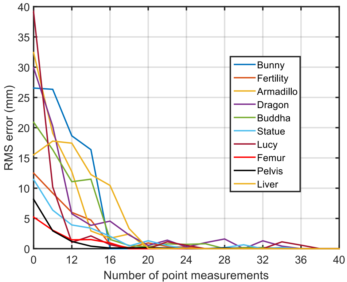
Figure 8-4: Plot of RMS error vs number of points used for registration, when using dSPR. For each integer element on the X axis, mean error is computed over 100 experiments. Most of the shapes considered need \approx 20 measurements for accurate registration.
