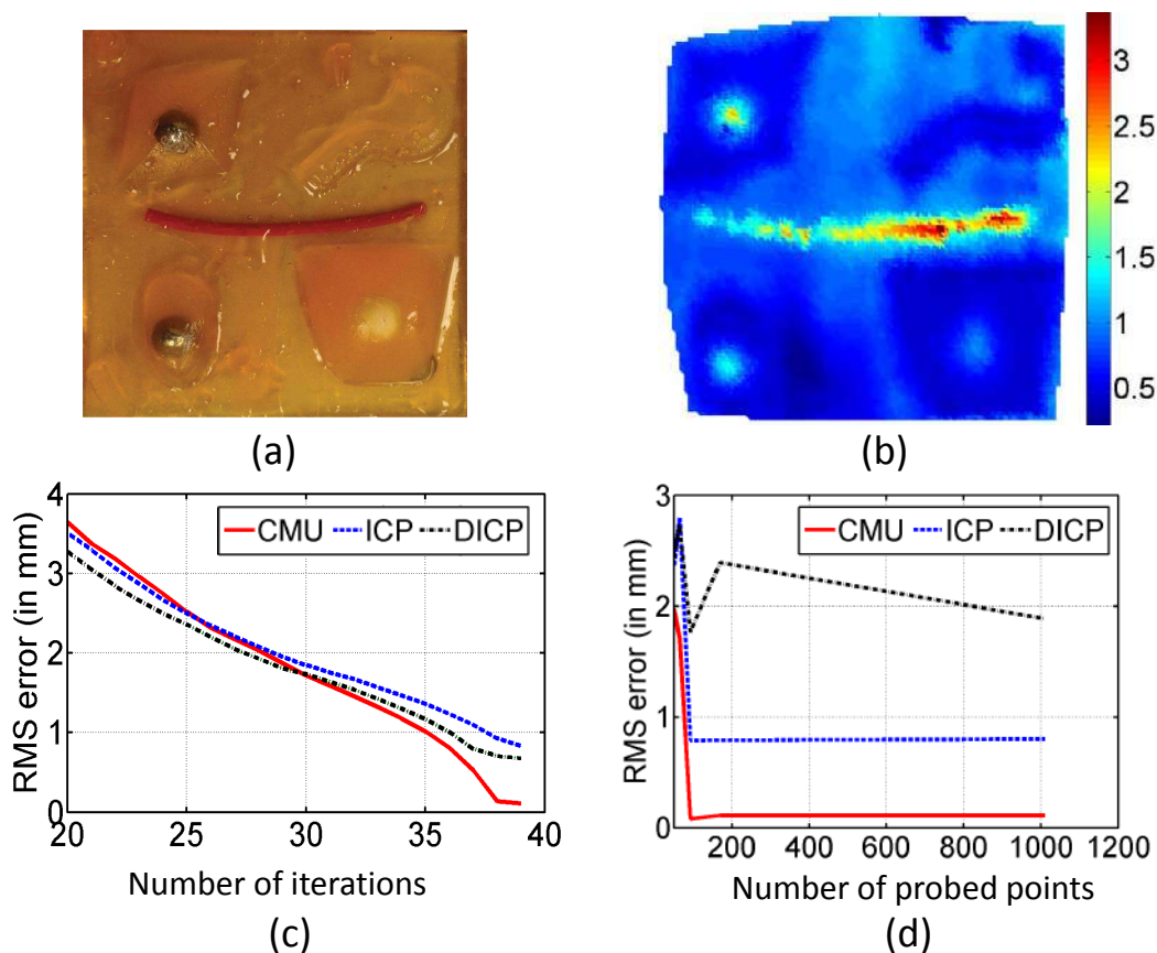
Figure 3-6: (a) Top view of the silicone organ (b) Stiffness map as estimated by SCAR-LSQ-CMU (Stiffness in N/mm) (c) Comparison of RMS error vs number of iterations (d) Comparison of RMS error vs number of probed points
