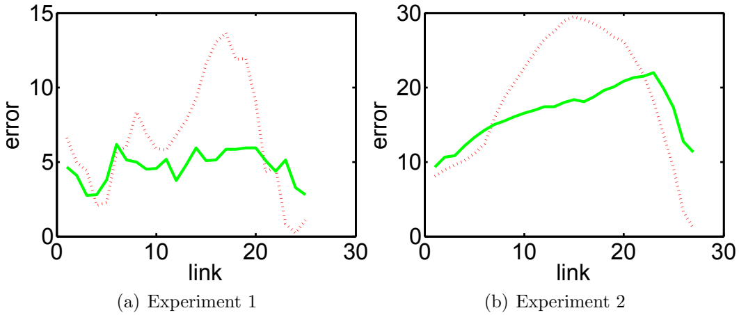
Figure 5-6: Comparison of variation in error between estimated position and ground-truth across the links. Green line is the variation using proposed approach and red dotted line is the variation using approach described by Tully et. al. [3]
