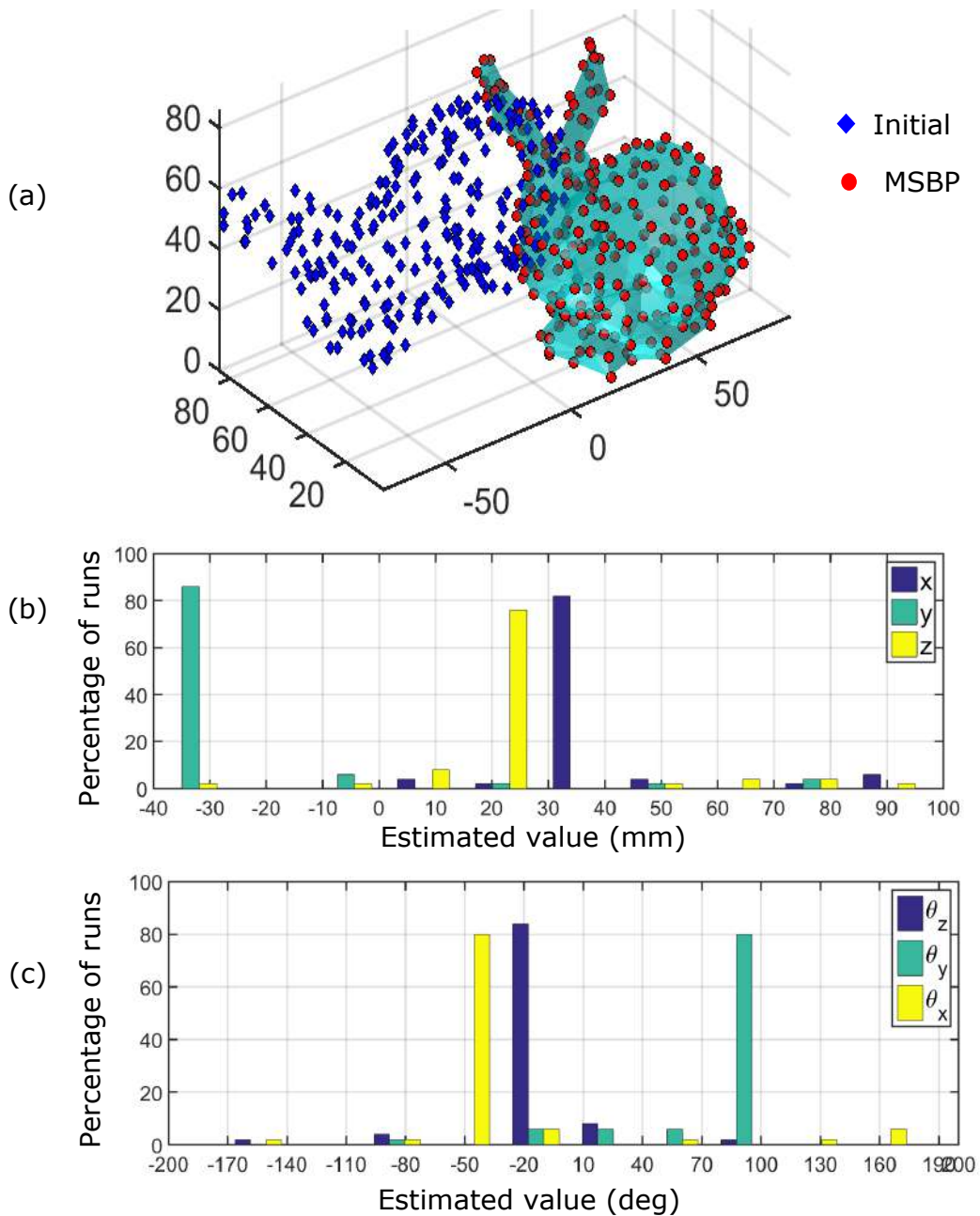
Figure 7-4: (a) CAD model of a Stanford bunny. The initial position of 1000 points is shown in blue-diamond markers, the position estimated by MSBP is shown in red-circular markers. (b) Histogram of the estimated translation parameters, (c) histogram of the estimated rotation parameters over 100 runs of the algorithm. In (b) and (c), the Y axis shows the percentage of runs that return a particular value and the X axis shows the estimated value returned by the parent state with the smallest innovation. MSBP has a high success rate of estimating the optimal parameters.
