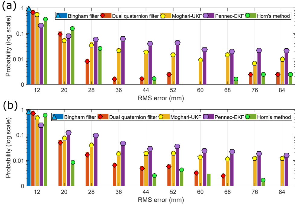
Figure 6-5: Histogram shows the RMS errors for the Bingham filter (BF), dual quaternion filter (DQF) from Chapter 4, unscented Kalman filter of [5] (Moghari-UKF), extended Kalman filter of [6] (EKF) and an incremental variant of Horn’s method ([4]). (a) The results shown are for Expt. 3, where the sensed points have a noise uniformly drawn from [-10 \text{ mm } 10 \text{ mm}] . The BF is most accurate with an average RMS error of 10.30 mm and a 100% success rate. (b) The results shown are for Expt. 5, where the sensed points have a noise obtained from a Gaussian distribution \mathcal{N}(\mathbf{0}, \text{diag}(10, 10, 10)) . The BF is the most accurate with an average RMS error of 4.95mm and a 100% success rate.
