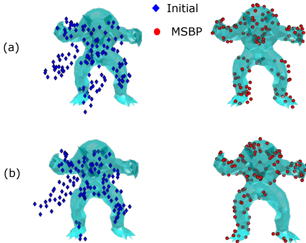
Figure 7-7: CAD model of a Stanford Armadillo man [7] and set of initial points sampled from parts of the model. The points are not sampled uniformly from all over the CAD, but have regions of missing information. (a) and (b) show two instances of incomplete data registered accurately to the CAD model using MSBP.
