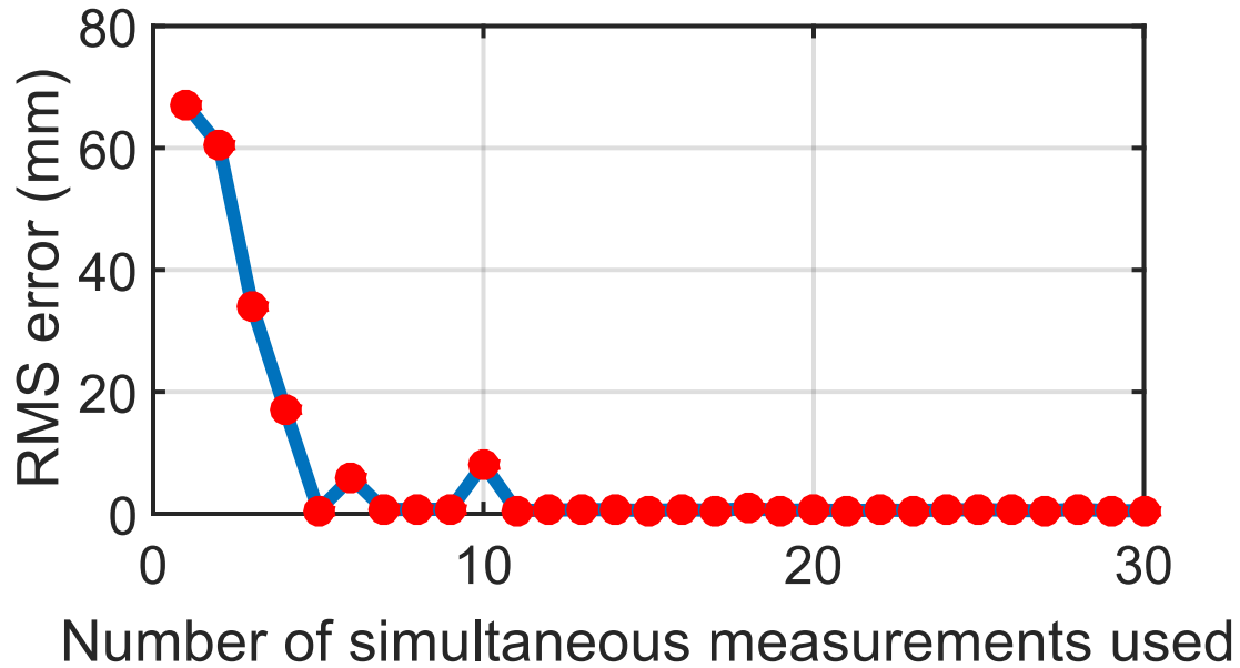
Figure 6-9: Plot shows RMS error upon convergence versus number of simultaneous measurements used. The more the number of simultaneous measurements used, the lower is the RMS error.
