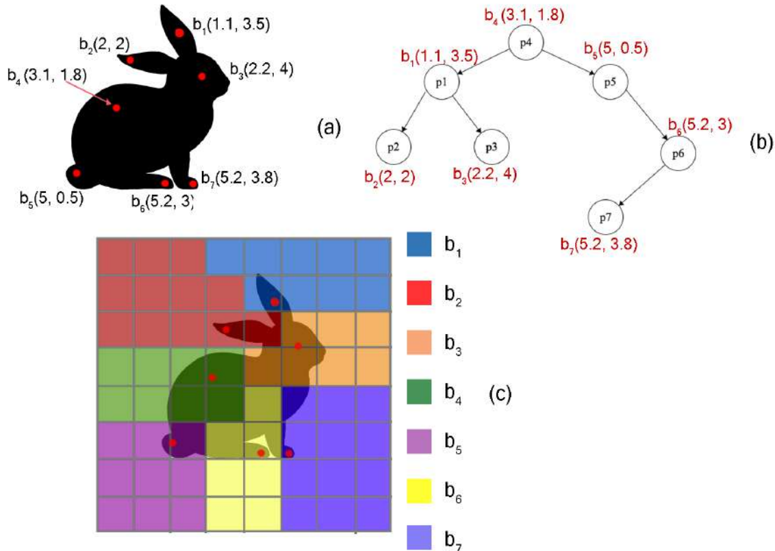
Figure 6-3: (a) Shows a representative point cloud of a model. For ease of demonstration, we show a 2D case. Let the model have 7 points as shown by red dots. (b) k -d tree constructed for the model points. (c) Look-up table approach is illustrated. A grid is created around the model. The closest point from each grid center to the model is computed using k -d tree. Each grid-color shows an index corresponding to the closest point on the model. Given a new sensor point, we first transform it to the model frame (using the best estimate of transformation). We then find which grid it belongs to and return the precomputed closest point.
