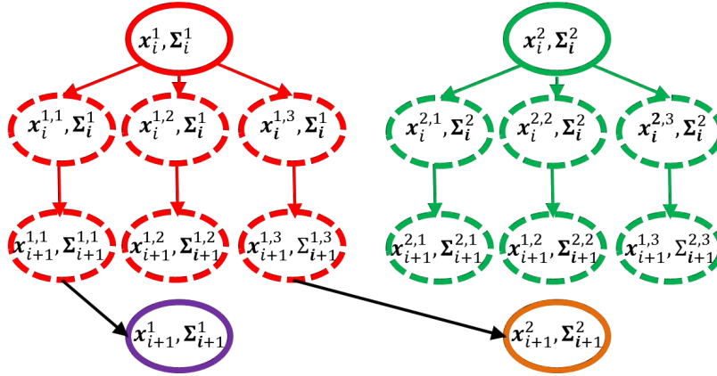
Figure 7-2: Steps involved in one iteration of the MSBP. Parent states are shown in bold ellipses and child states are shown in dashed ellipses. In this example, n = 2 , m = 3 .
