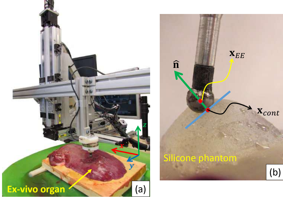
Figure 3-5: (a) Cartesian robot setup at Vanderbilt university used for experiments (b) Contact location and surface norm estimation
