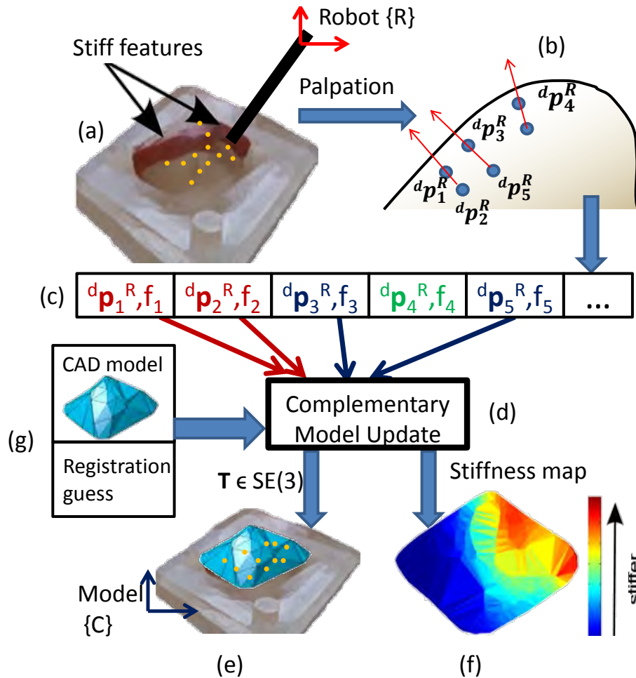
Figure 3-2: Flowchart describing the inputs and outputs for complementary model update (a) Flexible environment with embedded stiff features is probed by a robot (b) Location of probed points are sensed (c) Compatible force-position measurements are collected (d) complementary model update estimates the registration and stiffness map (e) Robot frame and model frame are registered (f) Stiffness map is generated (g) Prior geometric model and the initial registration guess
