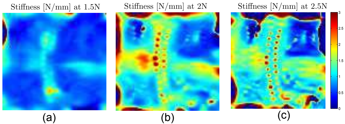
Figure 5-8: Representative stiffness distributions obtained at (a) f_2 = 1.5N , (b) f_3 = 2.0N and (c) f_4 = 2.5N .
