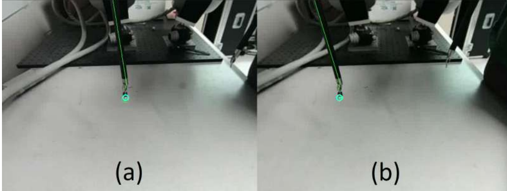
Figure 10-4: (a) and (b) are left and right camera views showing the dVRK robot tool. Cyan colored circles are drawn on both the images by finding the tool tip position from the robot kinematics and then using the registration between robot frame and camera frame. Note how the position of the circles visually confirms well with the true location of the tool tip.
