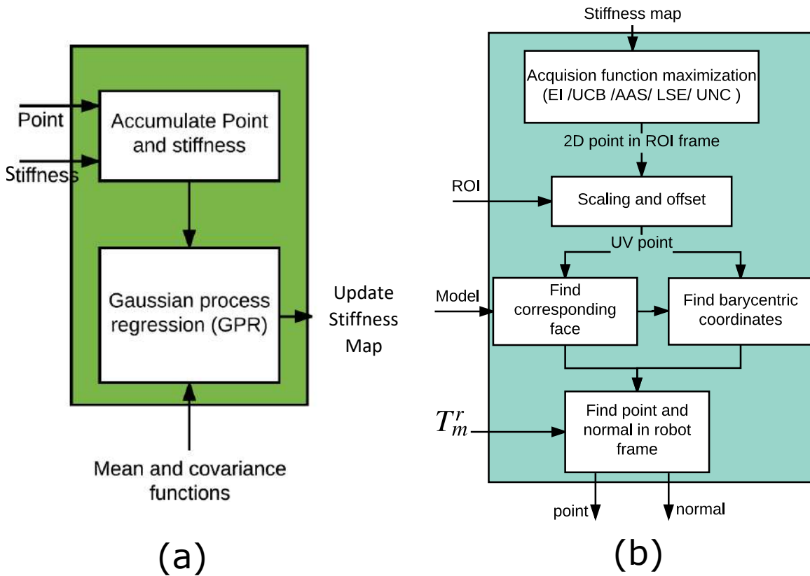
Figure 10-7: (a) An expanded flowchart of the “Stiffness map generation” block shown in Fig. 10-3. As the robot probes a new point on the organ, it calculates the stiffness value at that point. All the probed points with their corresponding stiffness values are accumulated and used to train a GPR (with predefined mean and covariance functions) which is used to updates the estimated stiffness map. (b) An expanded flowchart of the “Tumor search” block shown in Fig. 10-3
