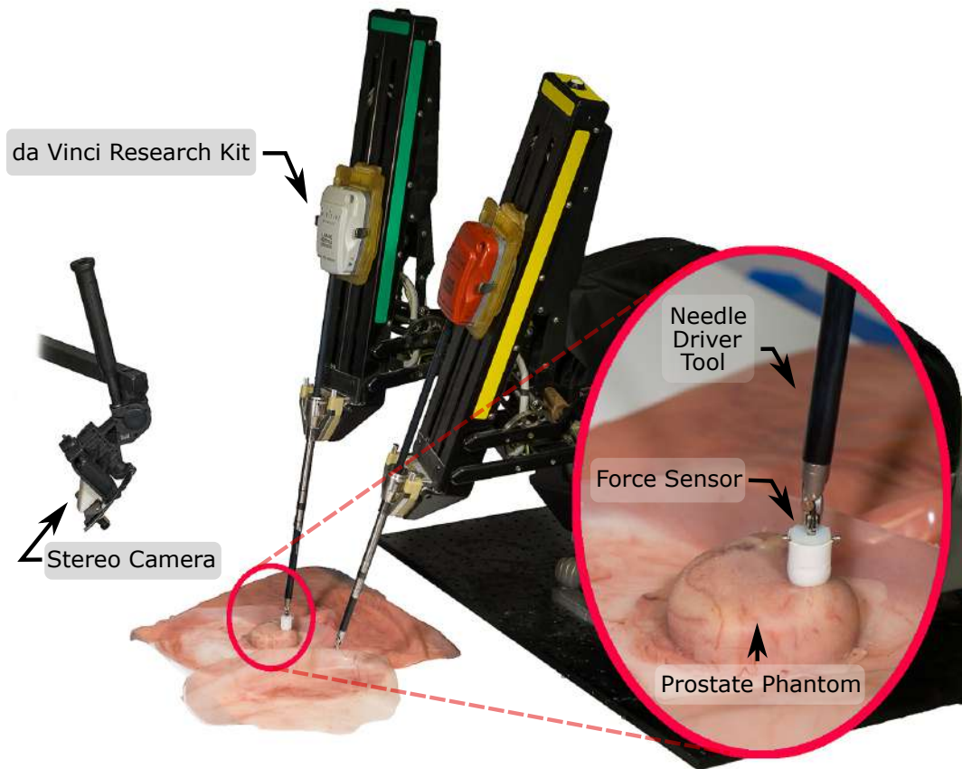
Figure 10-1: Experimental setup showing the dVRK robot with a miniature force sensor attached to the end-effector. A stereo camera overlooks the workspace of the robot. A phantom prostate with embedded stiff inclusion is placed in the workspace of the robot.
