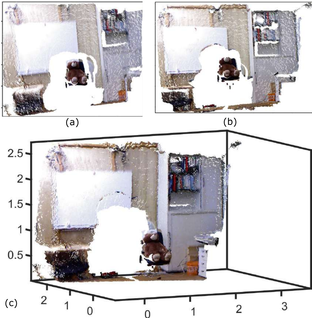
Figure 6-11: (a), (b), are two RGB-D images obtained from Kinect TM , with some overlapping region.(c) The point cloud model estimated by aligning the point clouds in (a) and (b) using the Bingham filter. The BF takes 0.21s to estimate the pose with an RMS error of 4.4cm, as opposed to ICP, which takes 0.46s with an RMS error of 6cm.
