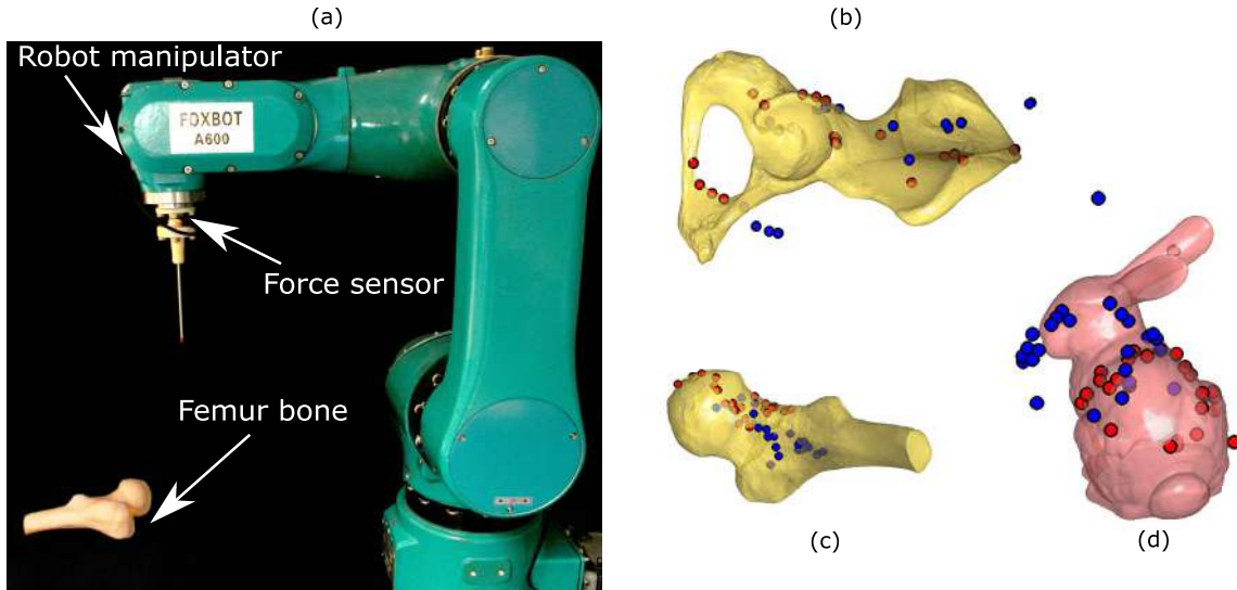
Figure 8-7: (a) Experimental set up consists of a robot manipulator equipped with a force sensor. The object that is to be registered is clamped and held in place. (b)-(d) Blue circles represent the initial location of the point measurements and red circles represent the registered location of the points. Pelvis bone, femur bone and bunny are probed at 18, 20 and 20 points respectively.
