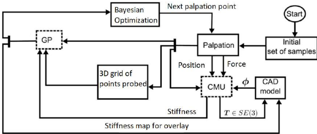
Figure 3-9: Block diagram description of the Bayesian optimization guided probing (Courtesy [2]).
