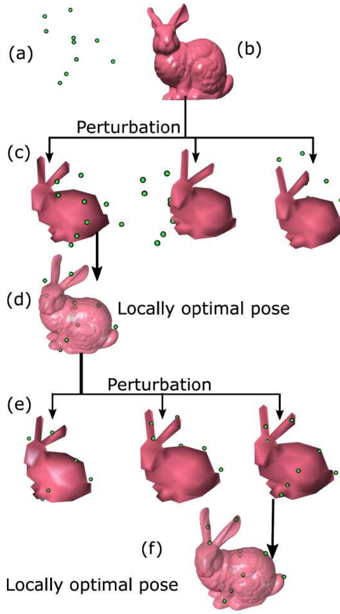
Figure 8-2: Figure shows the steps involved in an example of sparse point registration. In this example, two iterations of the algorithm are shown. The best pose estimate in each iteration is perturbed to obtain three pose particles. (a) Point measurements (b) Geometric model of the object (c) The geometric model in different perturbed poses. An approximate geometric model is used in this step. The number of triangle vertices in the original model is 259,896 and the number of vertices in the approximate model is 88. (d) The best pose from the perturbed poses is selected and a locally optimal pose is obtained by using ICP or bDQF and the original geometric model. (e) The best pose estimated from the previous iteration is perturbed to obtain three new poses. The perturbation in this step is lower than the previous iteration. (f) The locally optimal pose obtained after using ICP or bDQF. Note that the pose estimated in the second iteration provides an improvement over the previous iteration.
