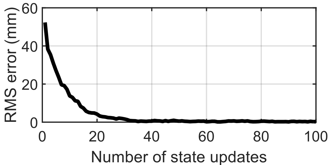
Figure 6-10: Plot shows the RMS error in the pose vs number of state updates as estimated by the Bingham filter using 20 simultaneous position and normal measurements in each update. The estimate converges in around 40 iterations.
