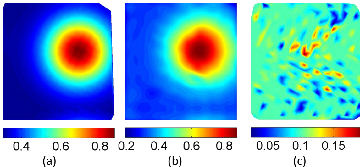
Figure 3-3: Stiffness in N/mm (a) Ground truth (b) Estimated by SCAR-LSQ-CMU (c) Estimated by SCAR-IEKF-old
