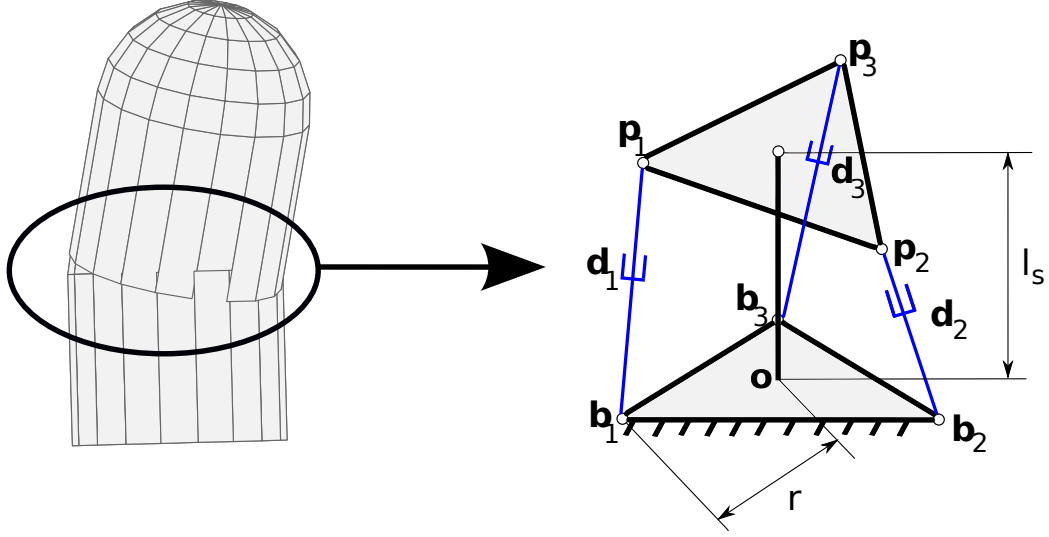
Figure 5-4: Kinematic representation of two adjacent links
