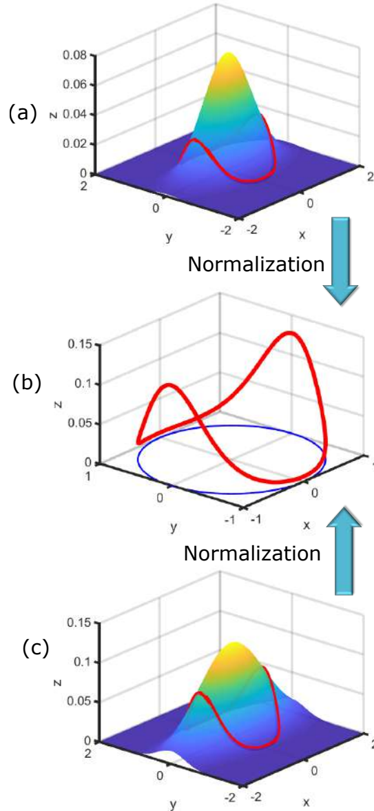
Figure 2-3: (a) A Gaussian distribution: f_1(\mathbf{v}) = \frac{1}{N_1} \exp(\mathbf{v}^T (\text{diag}(0, -3) - 1 \times \mathbf{I}_{2 \times 2}) \mathbf{v}) . In red is shown a slice of the Gaussian as made by points lying on a unit circle. (b) A Bingham distribution: f_2(\mathbf{v}) = \frac{1}{N_2} \exp(\mathbf{v}^T \text{diag}(0, -3) \mathbf{v}) . (c) A Gaussian distribution: f_3(\mathbf{v}) = \frac{1}{N_3} \exp(\mathbf{v}^T (\text{diag}(0, -3) - 0.5 \times \mathbf{I}_{2 \times 2}) \mathbf{v}) . In red is shown a slice of the Gaussian as made by points lying on a unit circle. The slice obtained from the Gaussian distributions in (a) and (c), when normalized result in the same Bingham distribution as shown in (b).
