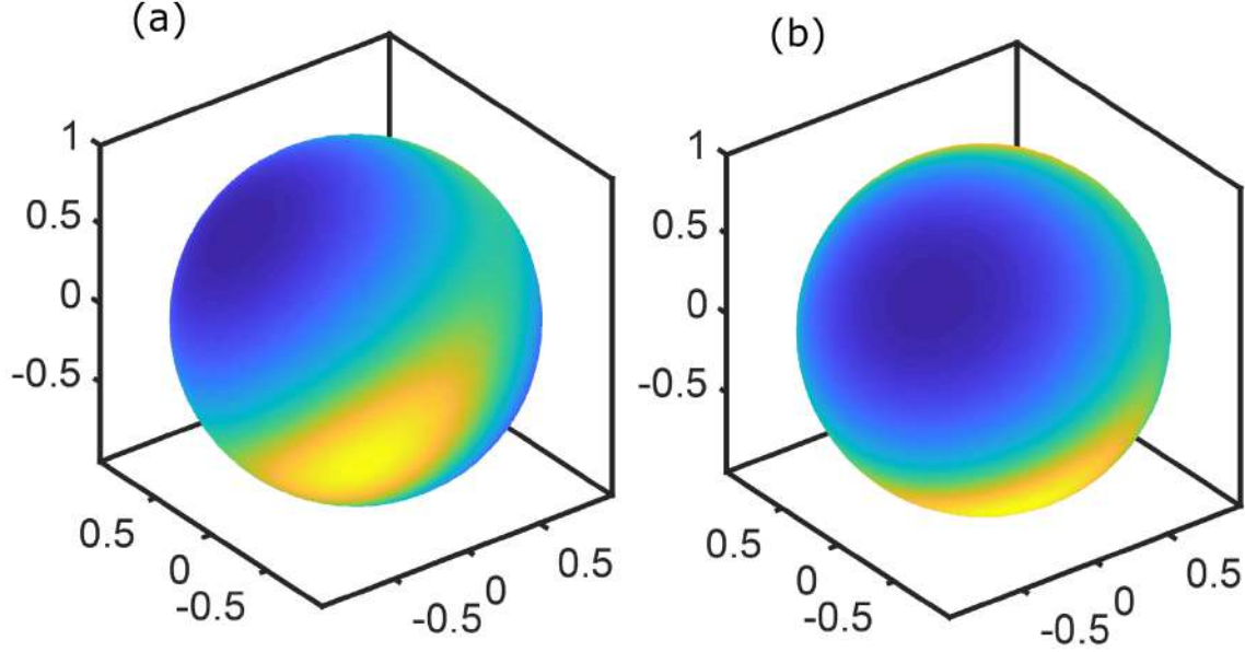
Figure 2-2: The figure shows two Bingham distributions with \mathbf{Z} = \text{diag}(0, -0.5, -2) , (a) \mathbf{M} = \begin{pmatrix} 0.5322 & -0.4953 & -0.6866 \\ 0.7747 & 0.6120 & 0.1591 \\ 0.3415 & -0.6166 & 0.7094 \end{pmatrix} , (b) \mathbf{M} = \begin{pmatrix} 0.2603 & -0.6941 & -0.6712 \\ 0.6578 & 0.6364 & -0.4029 \\ 0.7068 & -0.3366 & 0.6222 \end{pmatrix}
