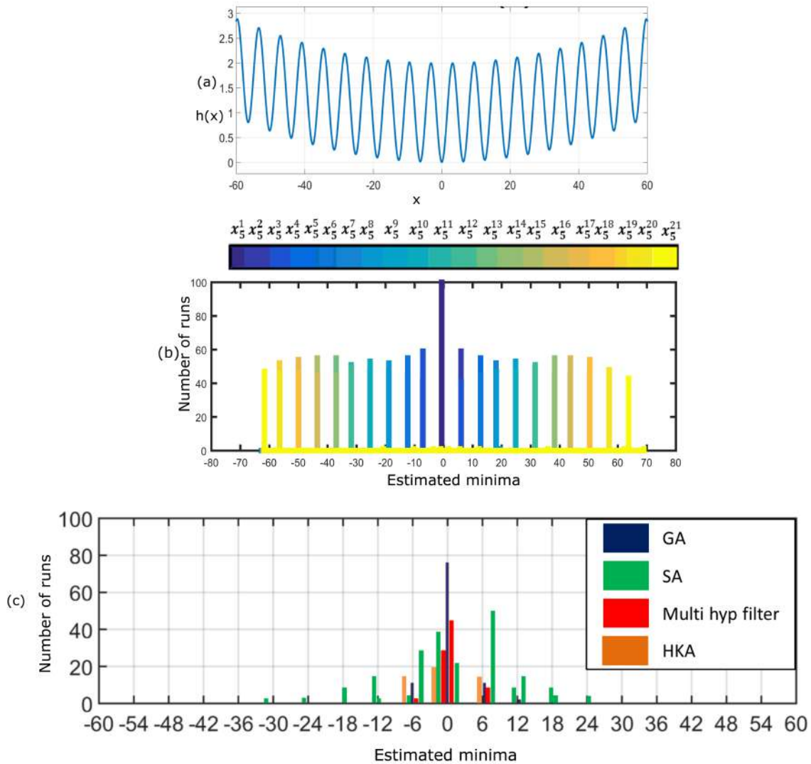
Figure 7-3: (a) A plot of the Griewank function. (b) A histogram showing the values estimated by 21 parent states of MSBP over 100 runs. The Y axis of the plot shows the number of runs that estimate a particular state and the X axis shows the estimated value. A histogram of the estimated value over 100 runs is shown for the following algorithms (c) Histogram showing values estimated by Genetic algorithm, Simulated annealing, Multi-hypothesis filter, and HKA.
