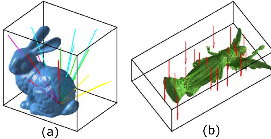
Figure 8-6: A cuboid is selected in the workspace of the robot that conservatively estimates the location of the object. (a) Different probing paths for the robot are selected such that the probed points are spread across the surface of the object. The colors of the path show the face of the cuboid that the paths originate from. (b) Point collection strategy for relatively flat object. Some paths do not produce a point on the object. If the robot does not make contact with the object during the course of its path, then the point is not included in the registration.
