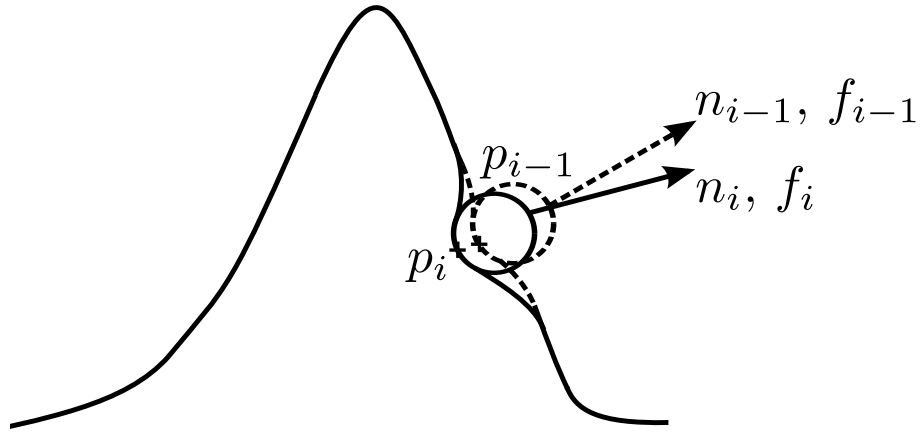
Figure 5-7: Schematic describing location of palpating points and the local surface normal at consecutive force scans.
