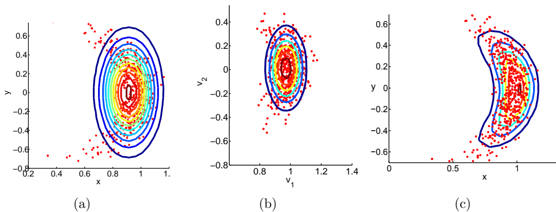
Figure 5-1: The red points show the final location of a differentially driven robot moving along a straight line, with noisy wheel speeds. The PDF contours of Gaussian of best fit (a) in Cartesian coordinates (b) in exponential coordinates (c) in exponential coordinates when mapped into Cartesian space.
