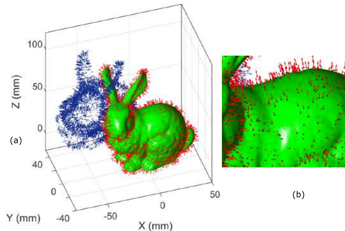
Figure 6-8: (a) Triangulated mesh of a Stanford bunny [7] is shown in green. Blue arrows represent initial location and red arrows represent estimated location of points and surface-normals. (b) Zoomed up view shows that the estimated location of points accurately rests on the triangulated mesh and the estimated direction of the surface-normals aligns well with the local surface normal. The Bingham filter takes 2.4s in MATLAB and 0.08s in C++ to estimate the pose.
