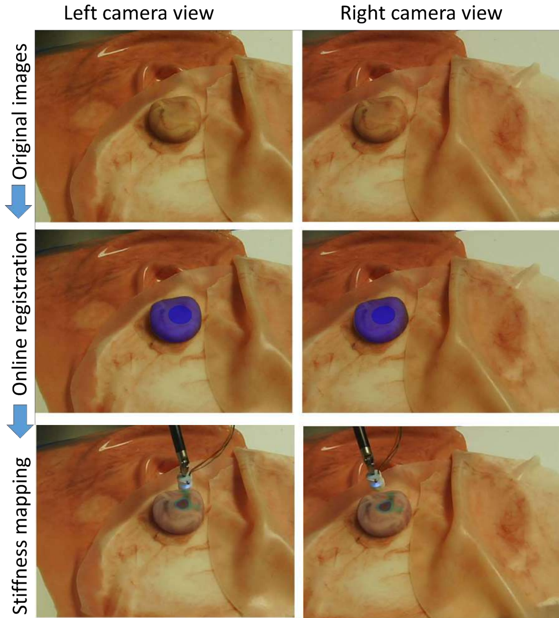
Figure 10-5: Top row: Original left and right camera images. Middle row: Camera images with registered prostate model shown in semi-transparent blue. The tumor model is also shown to allow us to compare our stiffness mapping result. Bottom row: The robot probes the organ and records force-displacement measurements. The estimated stiffness map is then augmented on the registered model in this figure. Dark blue regions show high stiffness. Note that the stiffness map reveals the location and shape of the tumor.
