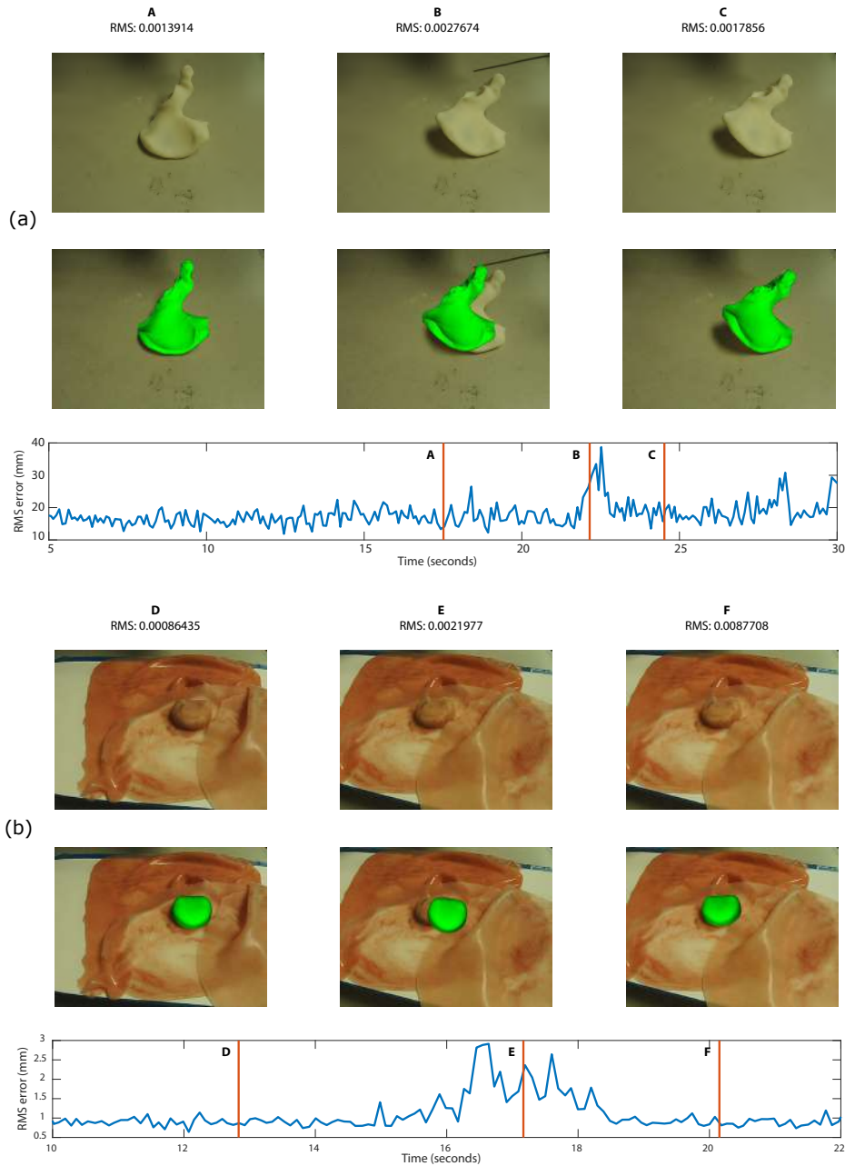
Figure 6-13: (a) Stereo image based tracking for a pelvis. Top row shows the left stereo camera image, middle row shows estimated pose superimposed and the bottom plot shows the RMS error vs time. At instance B, the pelvis was poked by the user which results in erroneous pose estimate. However, the pose estimate recovers to a low RMS error in a few seconds as shown in instance C. (b) Stereo image based tracking for a prostate. Top row shows the left stereo camera image, middle row shows estimated pose superimposed and the bottom plot shows the RMS error vs time. At instance E, the prostate is shifted by about 2 inches in less than a second, and the Bingham filter loses track of the object. However, the pose estimate recovers to a low RMS error in a few seconds as shown in instance F.
