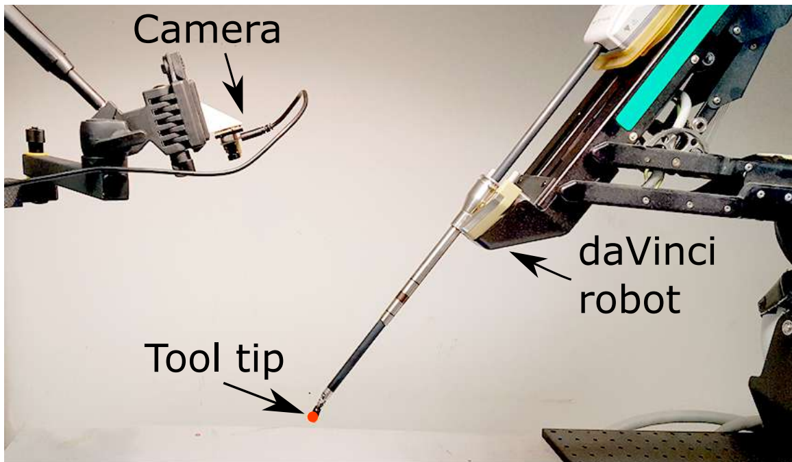
Figure 6-6: A spherical tool tip is attached to the daVinci robot. The tip is tracked using a stereo camera, which is held in a fixed position. As the robot is telemanipulated, the spherical tool-tip is tracked using the stereo camera, and the relative pose between the camera frame and the robot frame is estimated.
