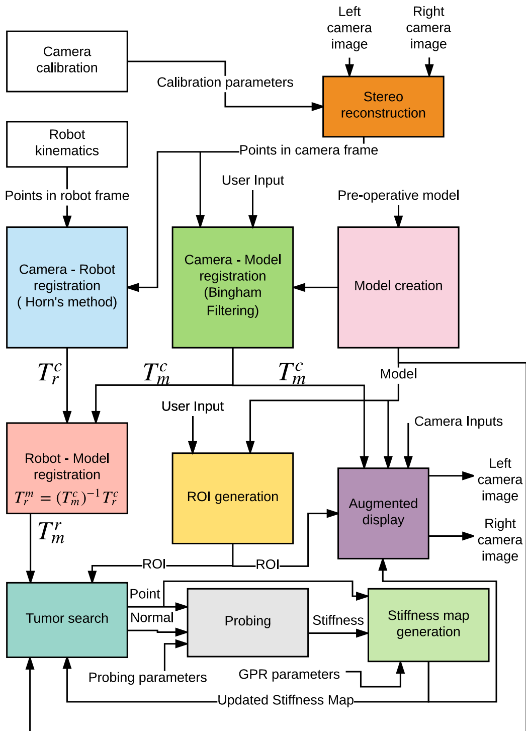
Figure 10-3: Flowchart showing all the modular components of our system. Some of the modules such as camera calibration, stereo reconstruction, model creation, and camera-robot-model registrations are performed once before the start of the experiment, while the other modules are constantly run for the duration of the experiment.
