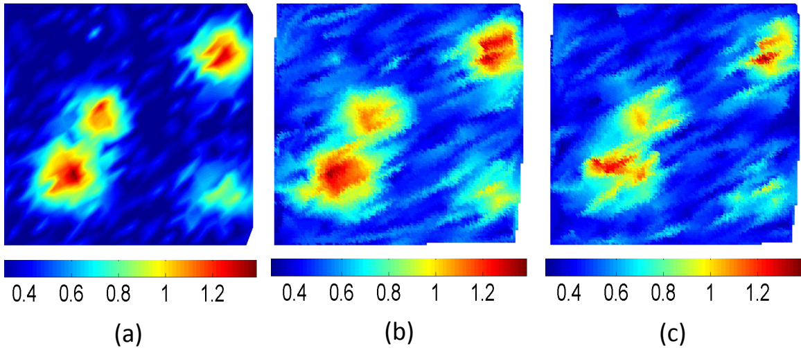
Figure 3-4: Stiffness in N/mm (a) Ground truth (b) Estimated under low sensor noise (c) Estimated under high sensor noise
