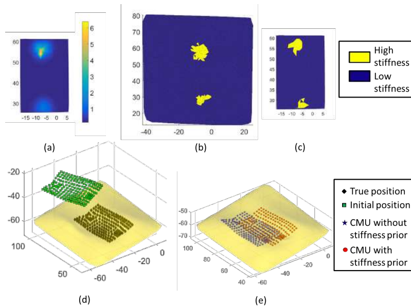
Figure 3-10: (a) Estimated stiffness map (stiffness in N/mm). (b) and (c) Prior stiffness map and estimated stiffness map respectively, normalized and stiffness values classified to high and low stiffness levels. (d) Initial and true location of probed points. (e) Estimated location probed points.
