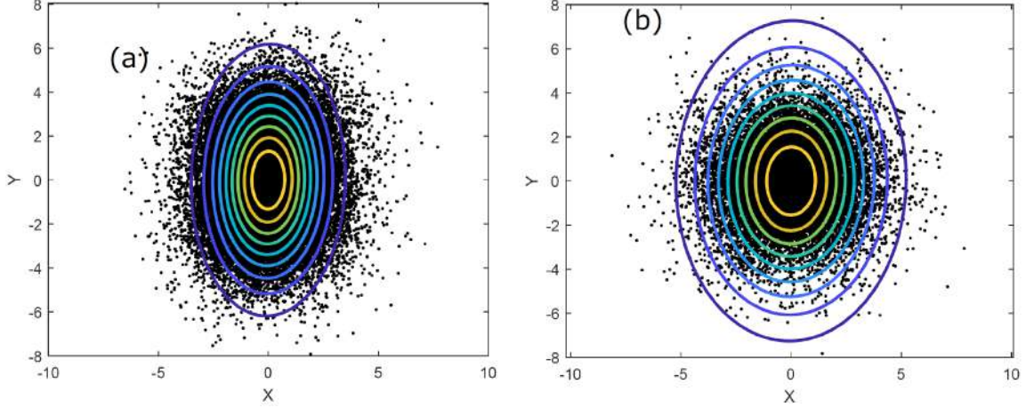
Figure -2: PDF contours obtained from the covariance estimated using Proposition 1. The black points are samples of \mathbf{h} = \mathbf{G}(\mathbf{x})\mathbf{b} + \mathbf{c} obtained from 100,000 Monte Carlo simulations. (a) \mathbf{Z} = \text{diag}(0, -30) (b) \mathbf{Z} = \text{diag}(0, -3) .
