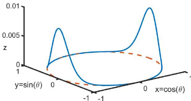
Figure 2-1: A 2D Bingham distribution: z = \frac{1}{N} \exp(\mathbf{s}^T \mathbf{M} \mathbf{Z} \mathbf{M}^T \mathbf{s}) , where \mathbf{M} = \mathbf{I}_{2 \times 2} , \mathbf{Z} = \text{diag}(0, -10) , and \mathbf{s} = (x, y) . The mode is at x = \pm 1, y = 0 .
