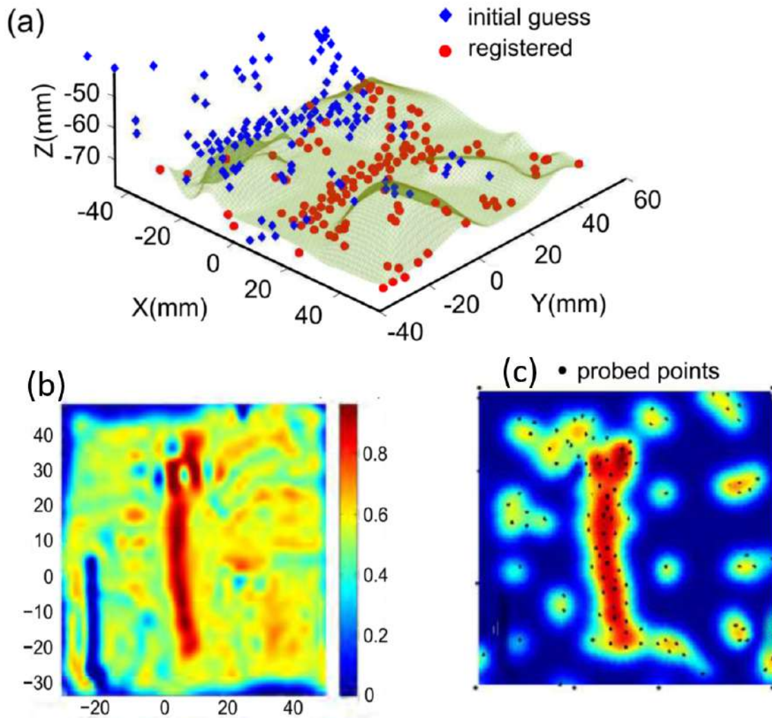
Figure 3-8: (a) Registration results for Example 3, (b) Ground truth stiffness map (c) Estimated map for Example 3 with 119 probed points. The algorithm starts with an initial grid of 19 points: 4 corners and 15 uniformly spaced points.
