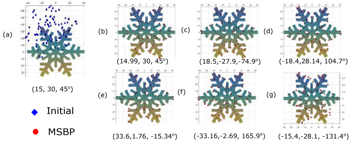
Figure 7-5: (a) CAD model of a snowflake. The initial position of 100 points and the position estimated by MSBP are shown in blue-diamond and red-circular markers respectively. The actual transformation between the points and the CAD model is (15, 30, 45^\circ) . (b)-(g) The first six parent states of MSBP. The estimated registration parameters are given below the figure. Note how the rotation angles are 45^\circ \pm n \times 60^\circ , ( n = 0, 1, 2 ) due to the 6 way symmetry in the shape of the snowflake. Snowflake CAD model courtesy of Thingiverse CAD model repository
