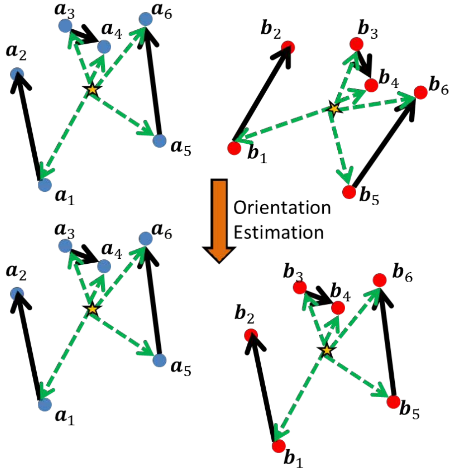
Figure 6-2: Blue points (left) indicate \mathbf{a}_i and red points (right) indicate \mathbf{b}_i . Our approach constructs vectors \mathbf{a}_v^{ij} = (\mathbf{a}_i - \mathbf{a}_j) and \mathbf{b}_v^{ij} = (\mathbf{b}_i - \mathbf{b}_j) as shown by black arrows. The Bingham filter estimates the orientation between the black vectors. A standard implementation of Horn [4] on the other hand, finds the orientation between the green-dashed vectors. While the green-dashed vectors can only be constructed using a batch of measurements, the black vectors can be constructed from sequential measurements. The black vectors can be considered to be a special case of green-dashed vectors where one pair of data points are considered at a time with one of the points serving as the centroid.
