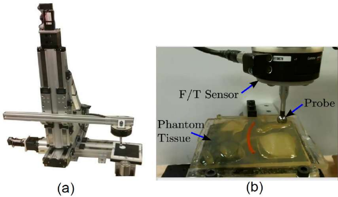
Figure 5-10: (a) 3-DOF Cartesian Robot at Vanderbilt University and (b) Experimental setup with the probe palpating the phantom tissue.
