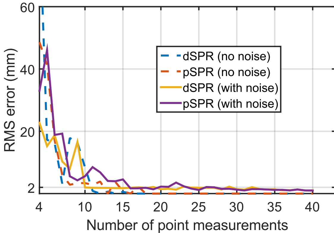
Figure 8-5: Plot of the RMS error vs number of measurements used for dSPR and pSPR, with a without noise in the measurements. In the absence of noise, dSPR takes 12 measurements and pSPR takes 18 measurements to converge to zero RMS error. In the presence of a uniform noise of 2mm, both pSPR and dSPR converge to an RMS error of < 2 mm after 20 measurements.
