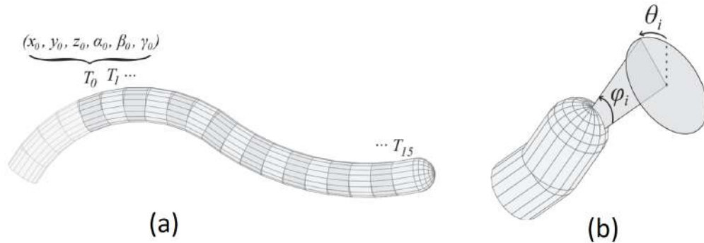
Figure 5-3: (a) The state parameterization used to define the configuration of the snake robot. (b) The effect of angles \theta_i and \phi_i on the pose between two successive links. The images are taken from [3].
