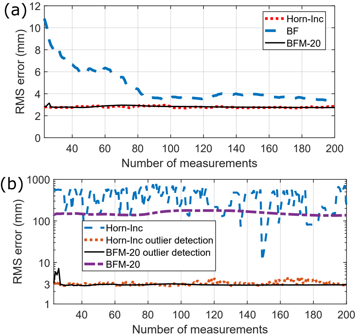
Figure 6-7: (a) Experimental results for robot-camera registration. BFM-20 produces the most accurate pose estimation, while Horn-Inc is the fastest and BF is the most erroneous. (b) Robot-camera registration results in the presence of 16% measurement outliers. In the absence of outlier detection both BFM-20 and Horn-Inc perform poorly. Outlier detection improves both BFM-20 and Horn-Inc, with the BFM-20 being smoother and more accurate.
