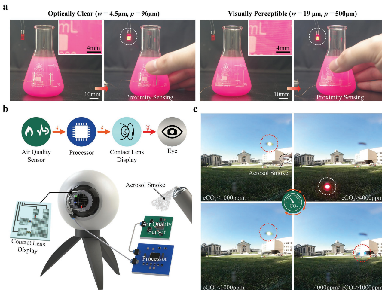
Figure 4. a) Proximity sensor using optically clear ( w = 4.5\ \mu\text{m} , p = 96\ \mu\text{m} ) and visually perceptible ( w = 19\ \mu\text{m} , p = 500\ \mu\text{m} ) conductor lines. b) Block diagram and schematic of air quality monitoring system composed of a contact lens display based on an LM circuit, an eyeball camera, an air quality sensor, and a microprocessor. c) Response sequence of air quality ( \text{CO}_2 ) measurement corresponding to “SAFE”-green, “DANGEROUS”-red, “ALEART”-blue and “SAFE”-green. LED coloring is set according to e\text{CO}_2 thresholds set at <1000\ \text{ppm} for “SAFE” and >4000\ \text{ppm} for “DANGEROUS.”
