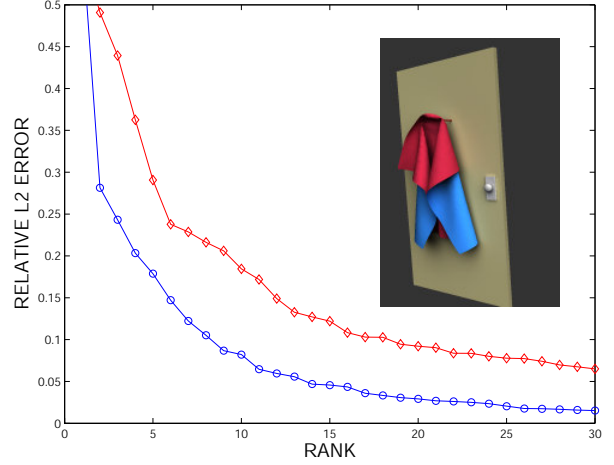
Figure 13: Model reduction : Relative l_2 error versus model rank, r_u and r_a , for the displacement (blue) and radiance transfer (red) models.
