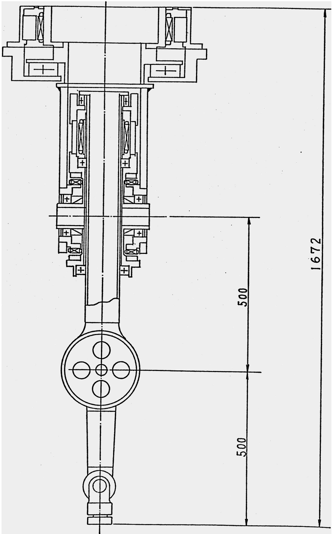
Figure 5: Drawing of CMU arm
