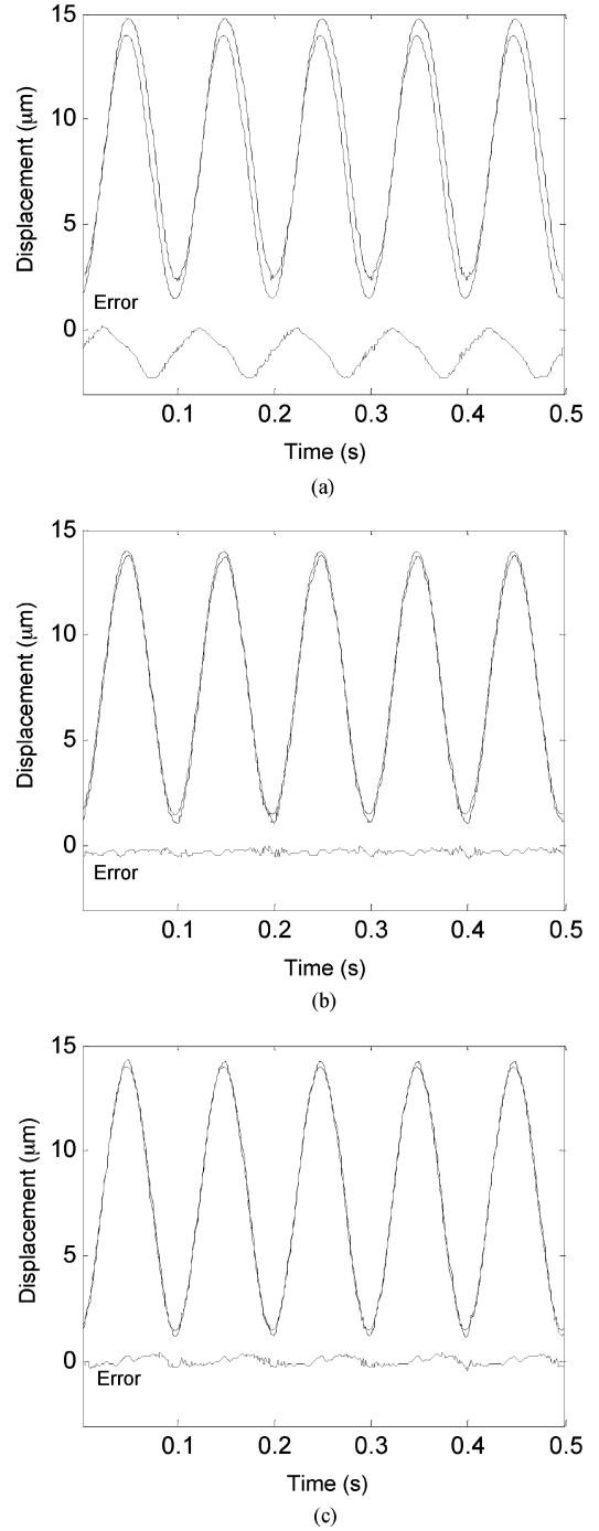
Fig. 10. Experimental open-loop tracking results of stationary 12.5- \mu\text{m} p-p sinusoids at 10 Hz. The rate-independent controller is based on the modified PI hysteresis model identified at the same 10-Hz, 12.5- \mu\text{m} p-p sinusoid. (a) Without controller. (b) Rate-independent controller. (c) Rate-dependent controller.
