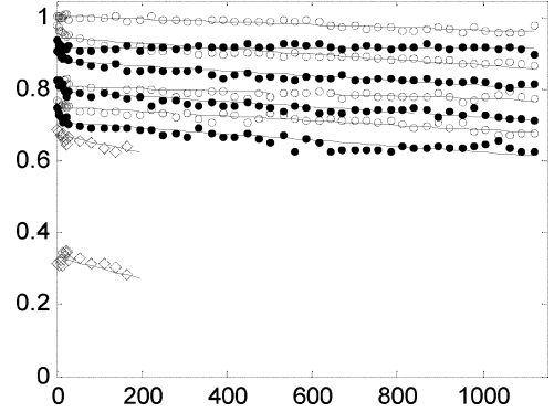
Fig. 8. Plot of the hysteresis slopes W_{hi} , i = 1 to 9, versus actuation rate \dot{x}(t) . Since the actuation rate is always slow at the turning points of a sinusoid, the first two sums of weights W_{h0} and W_{h1} are modeled up to 200\text{ }\mu\text{m/s} .
