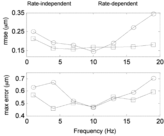
Fig. 9. Maximum errors and rms errors of the rate-independent and rate-dependent controllers in tracking 12.5- \mu\text{m} p-p stationary sinusoids at different frequencies. The rate-independent controller is based on the modified PI hysteresis model identified at the same 10-Hz, 12.5- \mu\text{m} p-p sinusoid.
