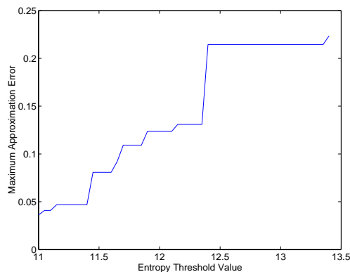
Figure 3. This is a plot of the maximum approximation error versus entropy threshold for the KL-divergence algorithm. (See the text for more details.)
