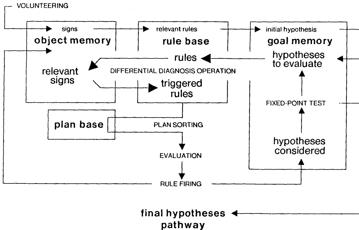
Figure 4-1: General mechanism of the NCLOSE algorithm
