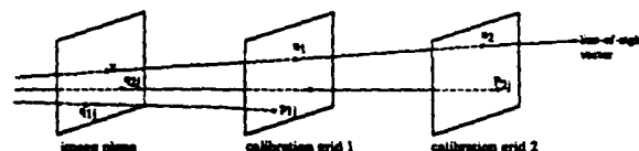
Figure 2: Two-Plane Calibration
