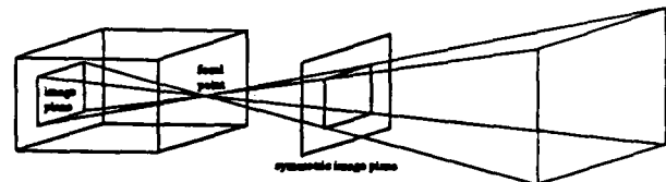
Figure 1: The Pinhole Camera Model
