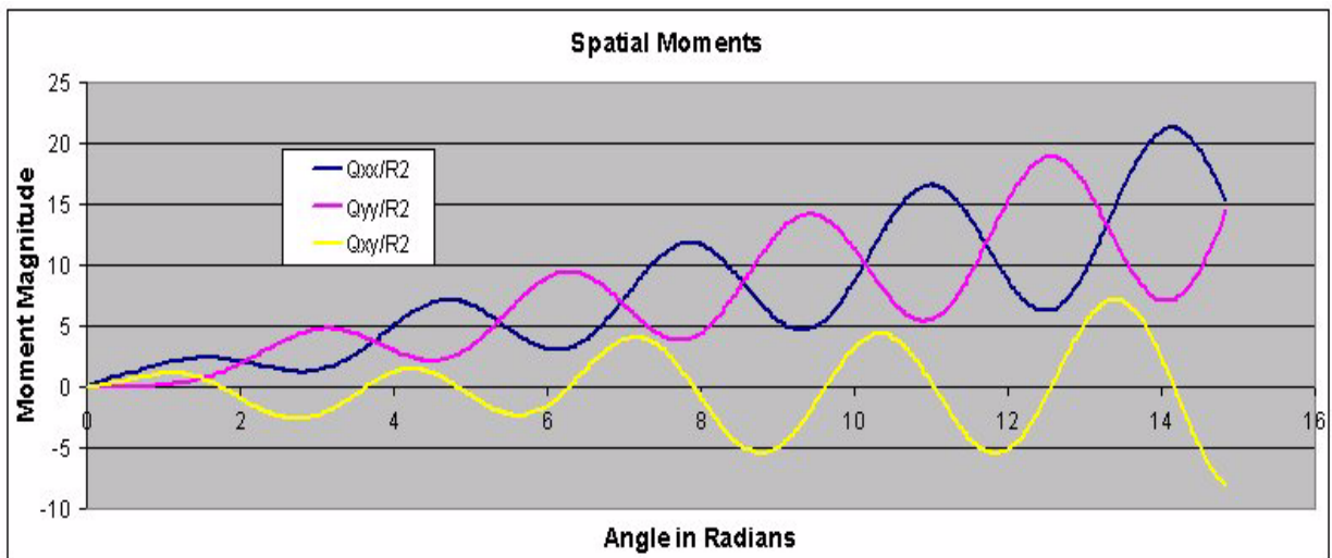
Figure 6 Spatial Moments
