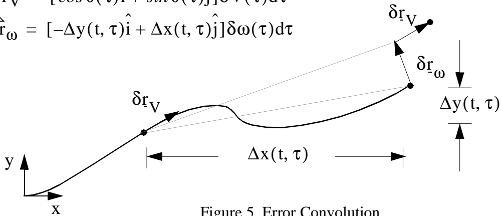
Figure 5 Error Convolution
