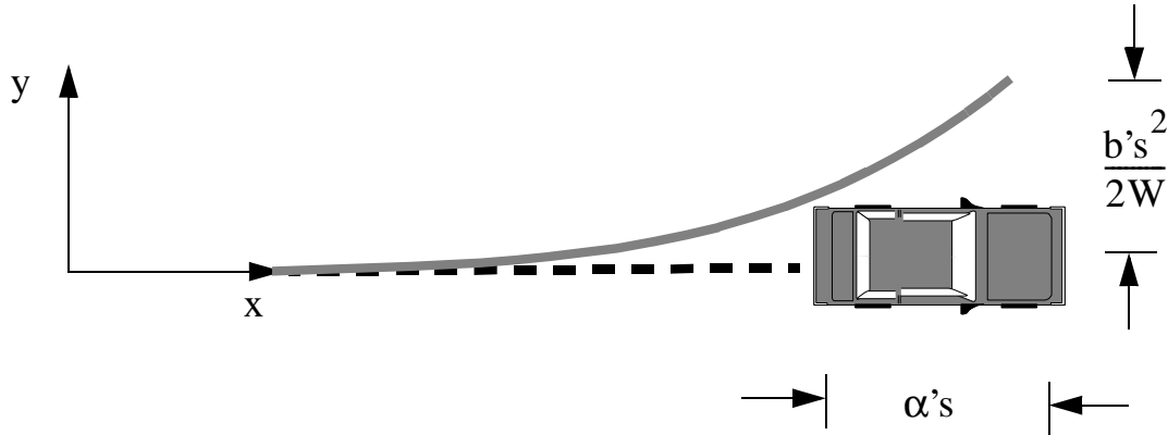
Figure 10 Differential Heading Odometry
