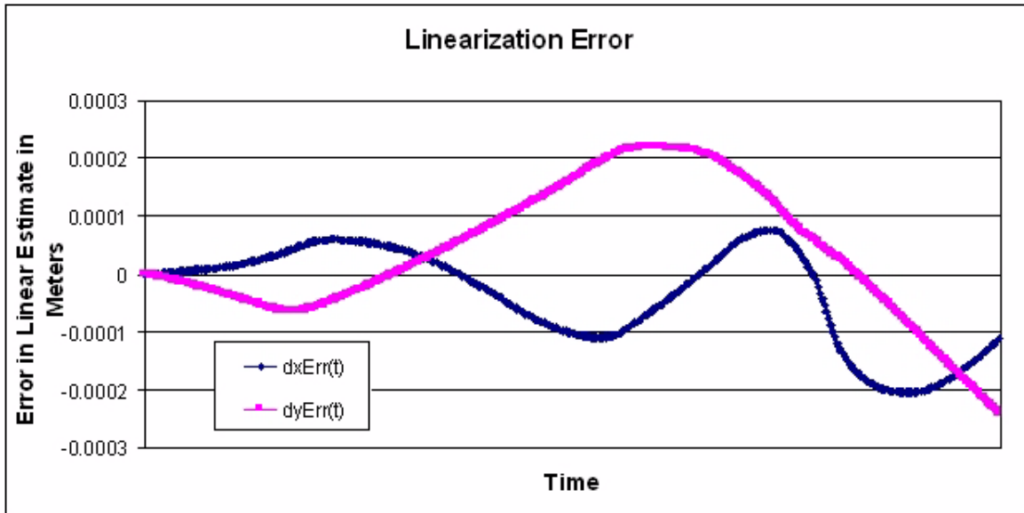
Figure 15 Simulated Integrated Heading Test Run Linearization Error
