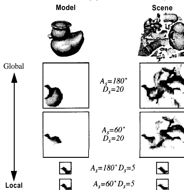
Figure 3. How spin-image generation parameters localize spin-images to reduce the effect of scene clutter and occlusion on matching.
