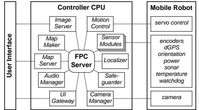
Figure 2. Controller architecture
