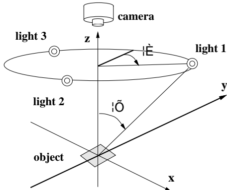
Figure 1: Arrangement for taking replica images under various direction light source.
