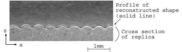
Figure 9: Comparison of reconstructed profile with actual cross section
