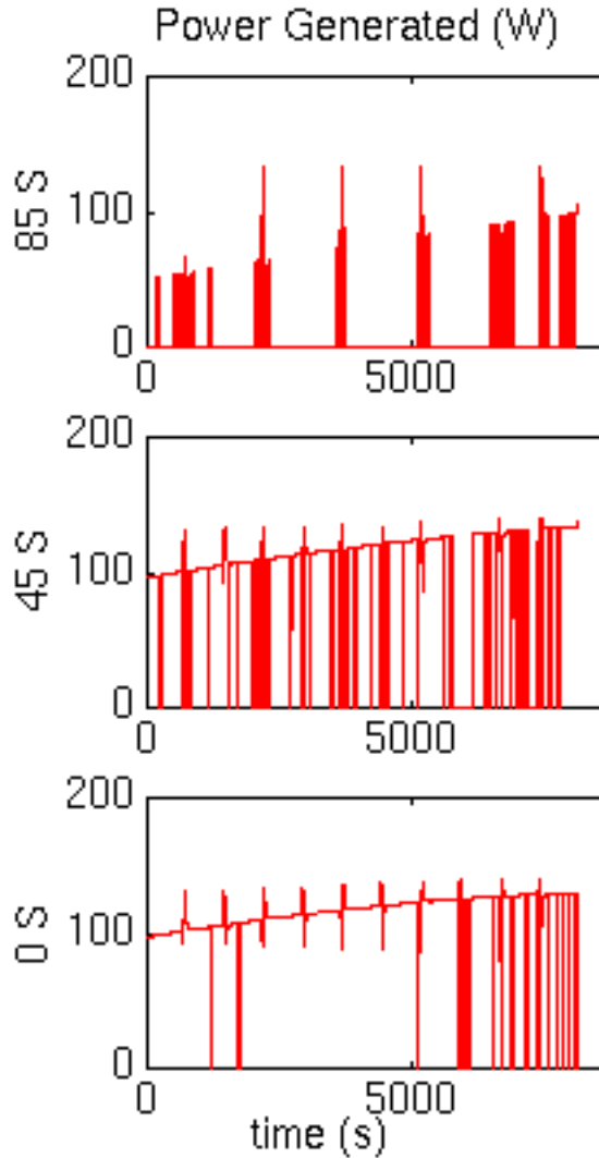
FIG. 6: Solar Power Generated within Crater
