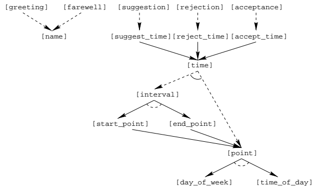
Figure 2: Fragment of a domain model for a scheduling task. A dashed edge indicates optional subconcept (default is required ), a dashed angle indicates inclusive subconcepts (default is exclusive ).
