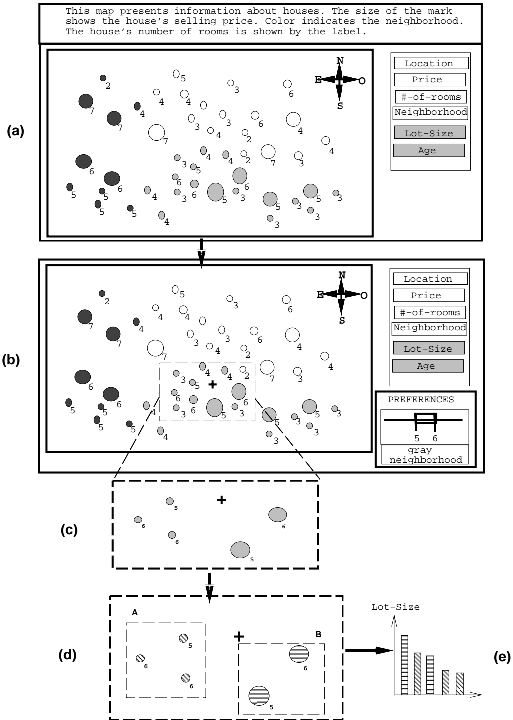
Figure 1: Sample IDEA system and sample Interaction.
