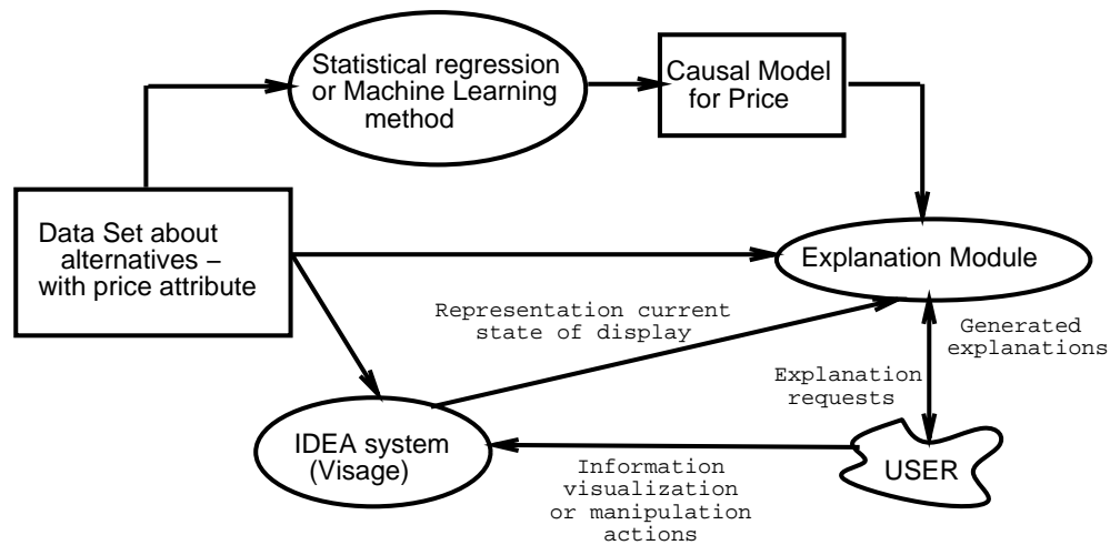
Figure 4: System architecture.
