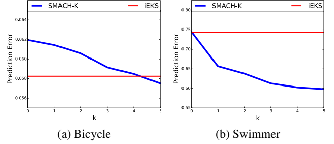
Figure 3: Performance of SMACH with respect to k (length of predictive states) for models with latent states.
