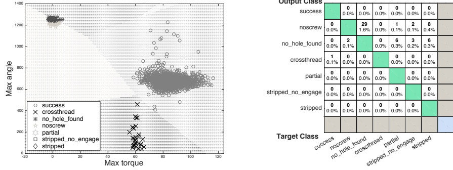
(a) Scatter plot of data overlaid on logistic regression classification regions
