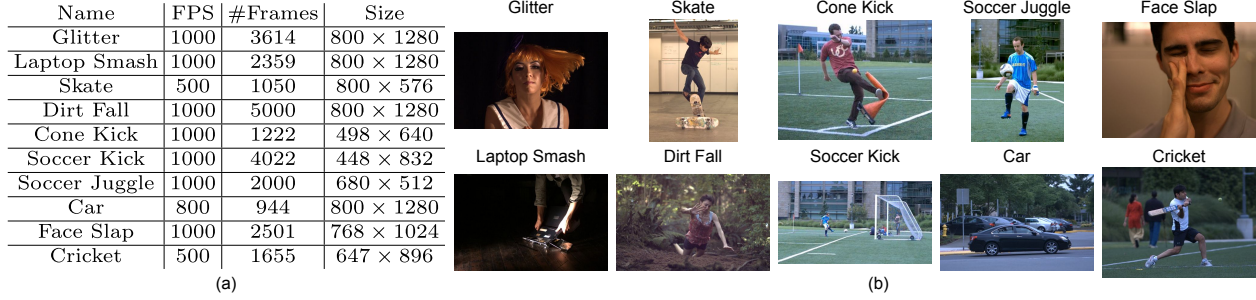
Figure 6. The high-speed video sequences used for experimental study. (a) Video statistics. (b) Key frames.
