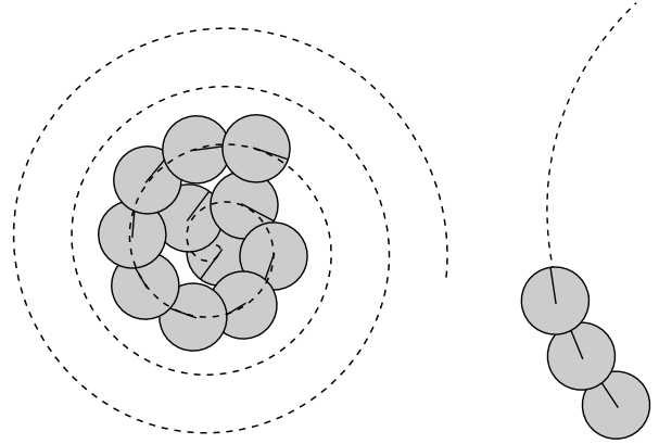
Fig. 4. Simulated robot drive modes. Left: ‘spiral’ (robot drives at constant velocity in an Archimedean spiral), right: ‘drive’ (robot drives at constant velocity and turn rate, producing a circular arc).
