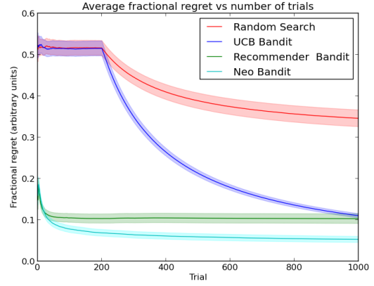
Fig. 6. Results for the indefinite horizon experiments. The solid lines represent the regret averaged over the test rooms the strategies were evaluated on. The shaded region represents a 95% confidence interval around that mean. The UCB bandit spends the first 200 trials examining the different state machines and is not significantly different from random search during that time. Once the bandit completes its initial exploration over the state machines its performance begins to converge towards the performance of the other bandit algorithms. The Recommender and Neo-Bandit algorithms both converge very quickly to a low average regret. The Neo-Bandit converges to a much lower average regret and with a tighter confidence interval. It is clear to observe that the Neo-Bandit is the superior algorithm to employ in this setting.
