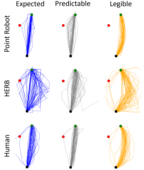
Fig. 7. The drawn trajectories for the expected motion, for \xi_P (predictable), and for \xi_L (legible).
