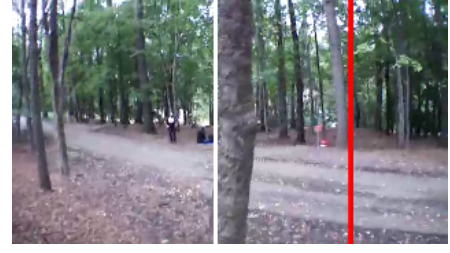
Fig. 2. One frame from MAV camera stream. The white line indicates the current yaw commanded by the current DAGger policy \pi_{n-1} while the red line indicates the expert commanded yaw. In this frame DAGger is wrongly heading for the tree in the middle while the expert is providing the correct yaw command to go to the right instead. These expert controls are recorded for training later iterations but not executed in the current run.
