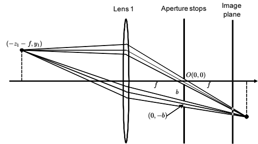
Fig. 5. Ray diagram of the multi-aperture telecentric imaging system. These stops are much larger than the actual size.
