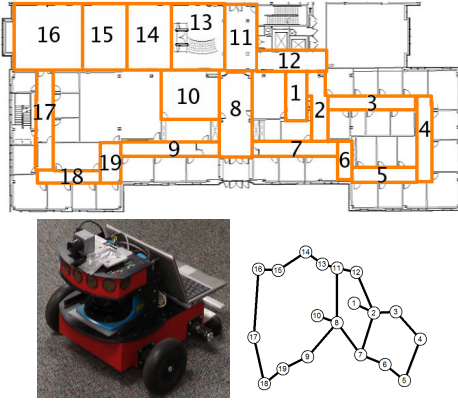
Fig. 4. Map of office building (top) used for experiments with a human/robot search team, and corresponding search graph (bottom right). Pioneer robot searcher (bottom left) with laser rangefinder and camera. The robot used the laser rangefinder for localization, and it used the camera to provide video feed to the humans. The robot and human team started at the entrance in cell 8.
