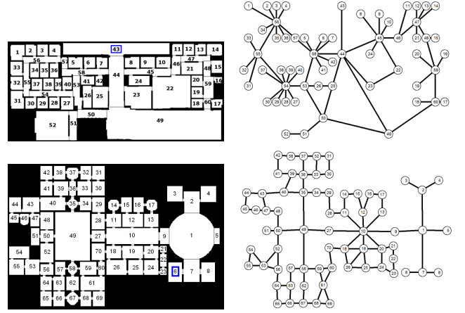
Fig. 2. Example floorplans (left) and graphical representations (right) of environments used for simulated coordinated search. The office (top) required three searchers to clear, and the museum (bottom) required five. Starting cells are denoted with a square.
