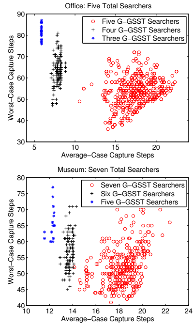
Fig. 3. Scatter plot of search schedules from the combined algorithm. Each data point represents a schedule generated by a different spanning tree input to Algorithm 3. The data point shapes are based on the allocation of searchers to the guaranteed and efficient search roles. The total searchers remains constant throughout the trials.
